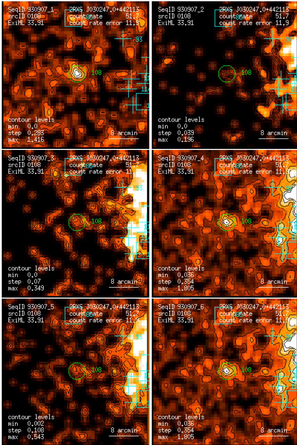
Figure 108: RASS 930907: detection 0108: band rate images, Gaussian filter: (1) PSPC channels 11 – 41, (2) 52 – 90, (3) 91 – 201, (4) 11 – 235, (5) 52 – 201, (6) 11 – 201. Broad band rates in counts/ks. Band rate contour levels in counts/ks/arcmin 2 .
