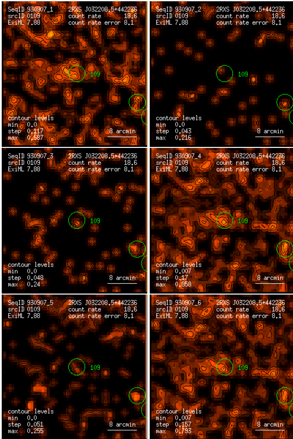
Figure 109: RASS 930907: detection 0109: band rate images, Gaussian filter: (1) PSPC channels 11 – 41, (2) 52 – 90, (3) 91 – 201, (4) 11 – 235, (5) 52 – 201, (6) 11 – 201. Broad band rates in counts/ks. Band rate contour levels in counts/ks/arcmin 2 .
