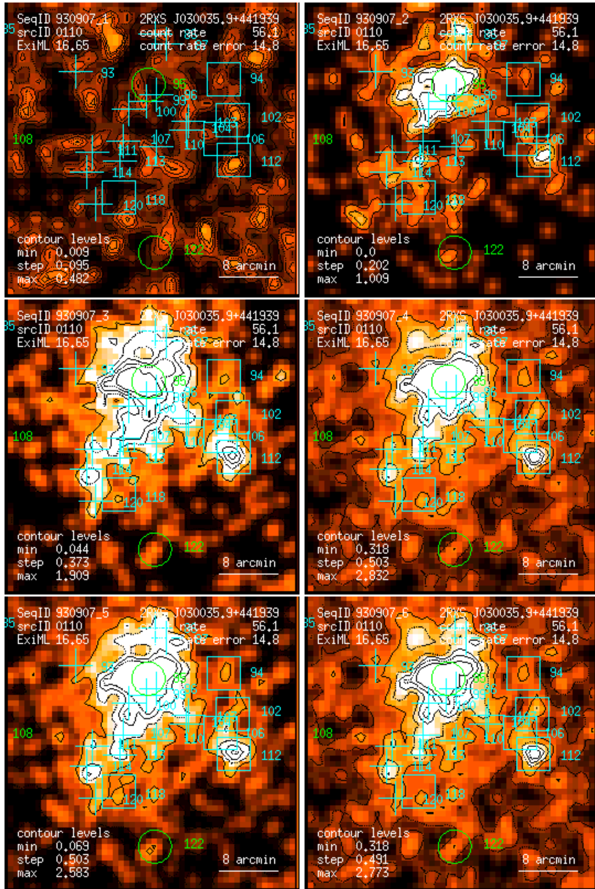
Figure 110: RASS 930907: detection 0110: band rate images, Gaussian filter: (1) PSPC channels 11 – 41, (2) 52 – 90, (3) 91 – 201, (4) 11 – 235, (5) 52 – 201, (6) 11 – 201. Broad band rates in counts/ks. Band rate contour levels in counts/ks/arcmin 2 .
