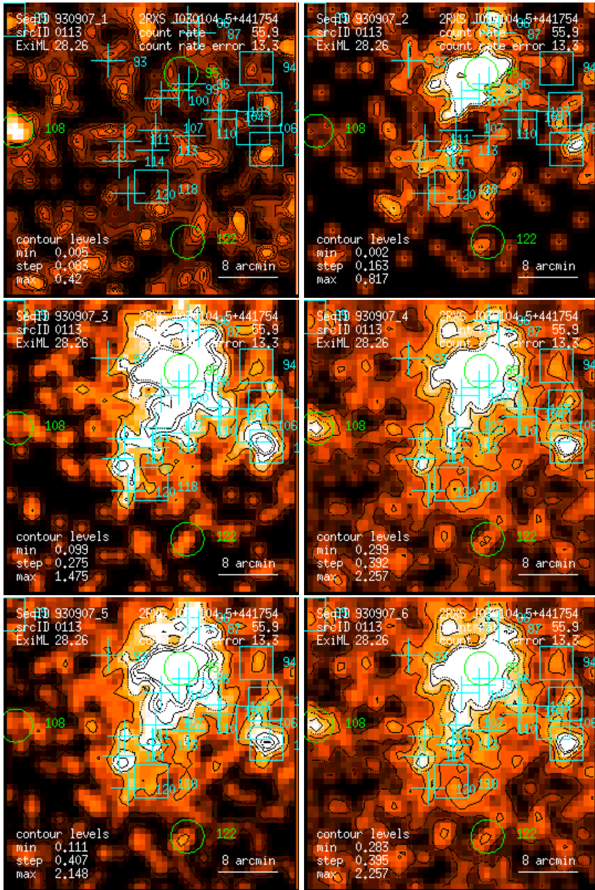
Figure 113: RASS 930907: detection 0113: band rate images, Gaussian filter: (1) PSPC channels 11 – 41, (2) 52 – 90, (3) 91 – 201, (4) 11 – 235, (5) 52 – 201, (6) 11 – 201. Broad band rates in counts/ks. Band rate contour levels in counts/ks/arcmin 2 .
