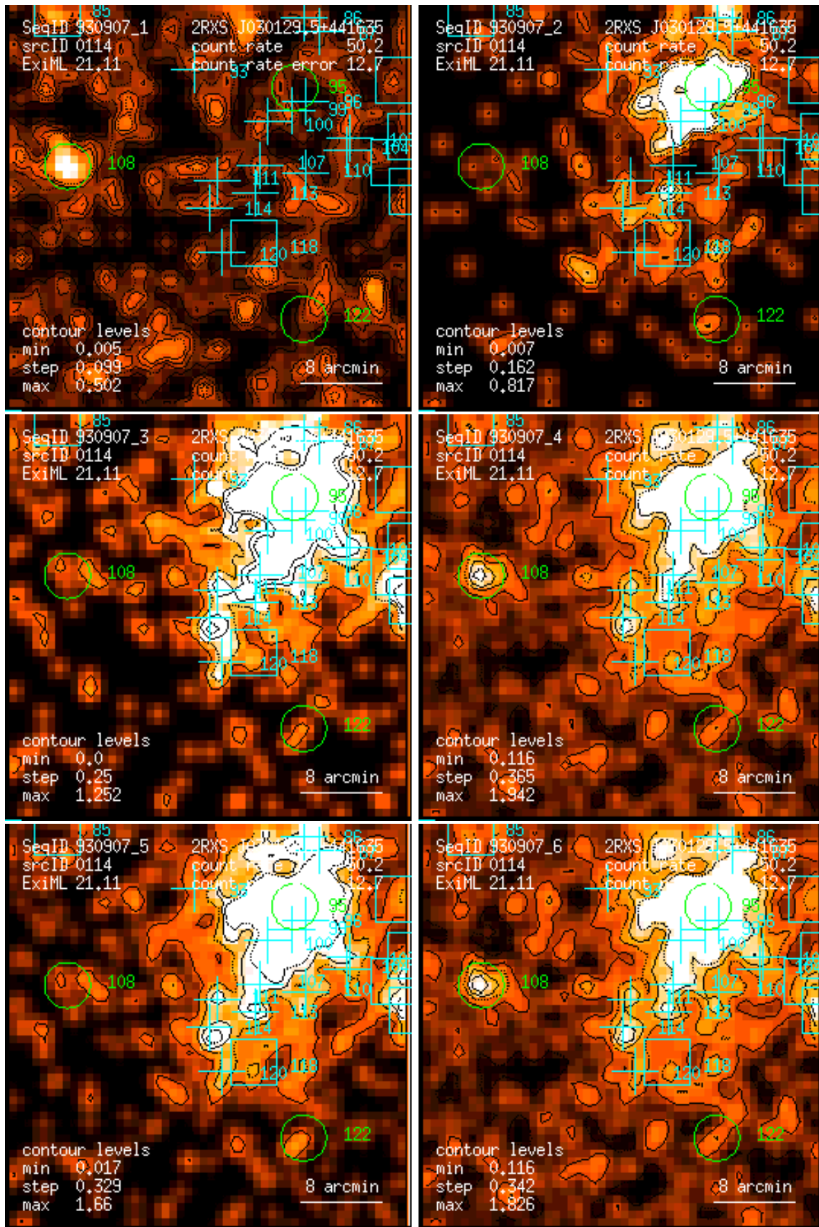
Figure 114: RASS 930907: detection 0114: band rate images, Gaussian filter: (1) PSPC channels 11 – 41, (2) 52 – 90, (3) 91 – 201, (4) 11 – 235, (5) 52 – 201, (6) 11 – 201. Broad band rates in counts/ks. Band rate contour levels in counts/ks/arcmin 2 .
