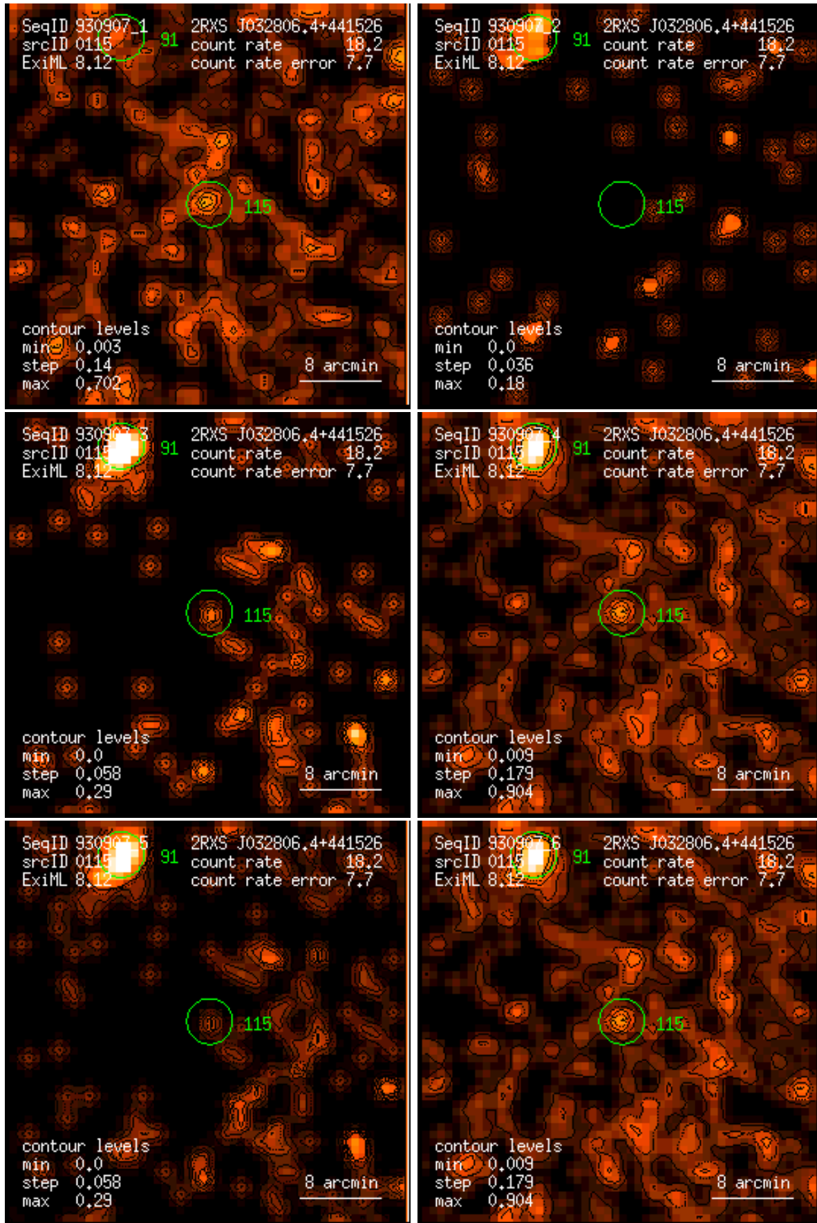
Figure 115: RASS 930907: detection 0115: band rate images, Gaussian filter: (1) PSPC channels 11 – 41, (2) 52 – 90, (3) 91 – 201, (4) 11 – 235, (5) 52 – 201, (6) 11 – 201. Broad band rates in counts/ks. Band rate contour levels in counts/ks/arcmin 2 .
