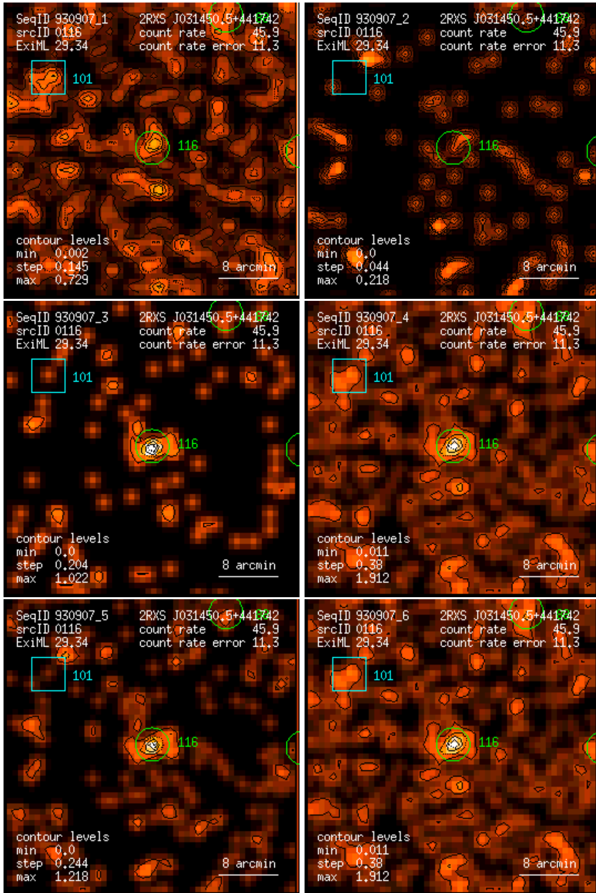
Figure 116: RASS 930907: detection 0116: band rate images, Gaussian filter: (1) PSPC channels 11 – 41, (2) 52 – 90, (3) 91 – 201, (4) 11 – 235, (5) 52 – 201, (6) 11 – 201. Broad band rates in counts/ks. Band rate contour levels in counts/ks/arcmin 2 .
