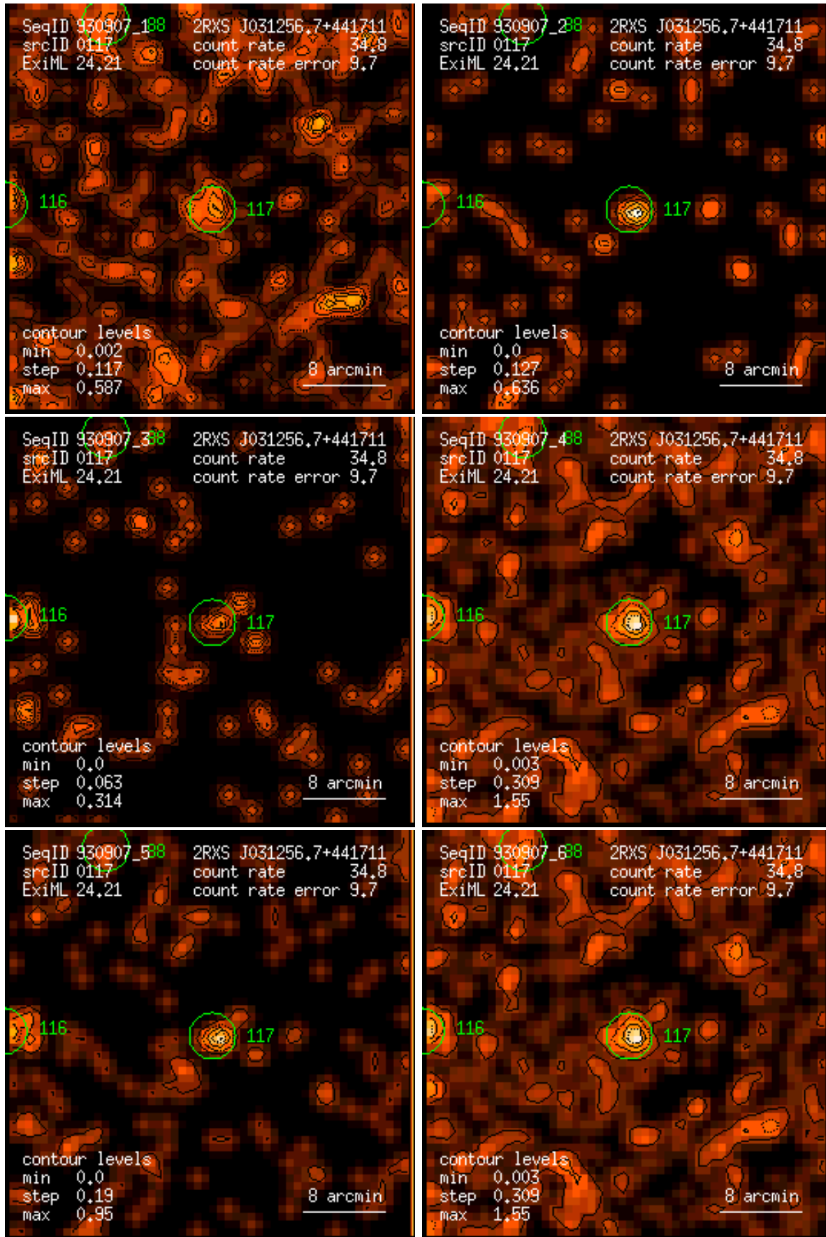
Figure 117: RASS 930907: detection 0117: band rate images, Gaussian filter: (1) PSPC channels 11 – 41, (2) 52 – 90, (3) 91 – 201, (4) 11 – 235, (5) 52 – 201, (6) 11 – 201. Broad band rates in counts/ks. Band rate contour levels in counts/ks/arcmin 2 .
