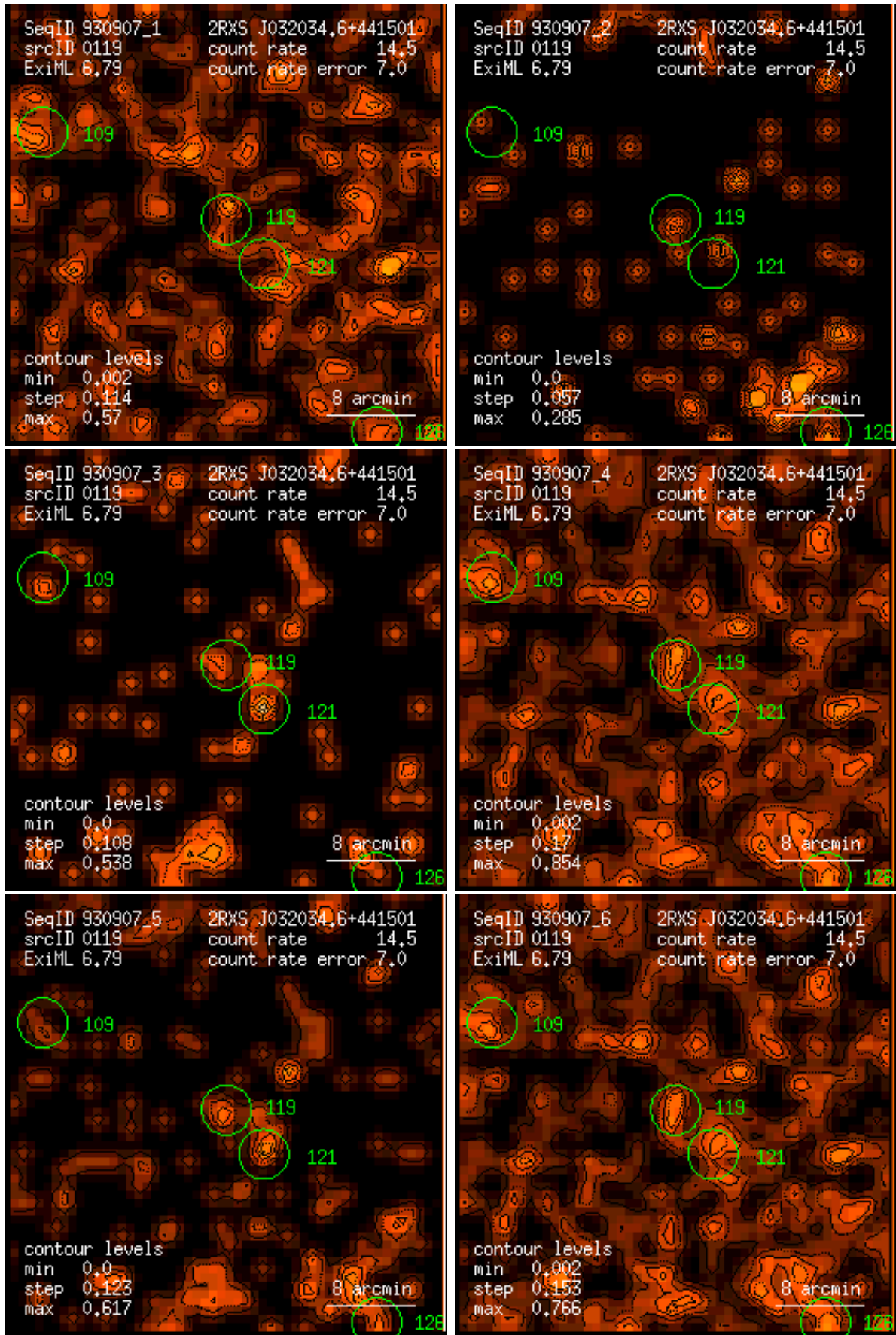
Figure 119: RASS 930907: detection 0119: band rate images, Gaussian filter: (1) PSPC channels 11 – 41, (2) 52 – 90, (3) 91 – 201, (4) 11 – 235, (5) 52 – 201, (6) 11 – 201. Broad band rates in counts/ks. Band rate contour levels in counts/ks/arcmin 2 .
