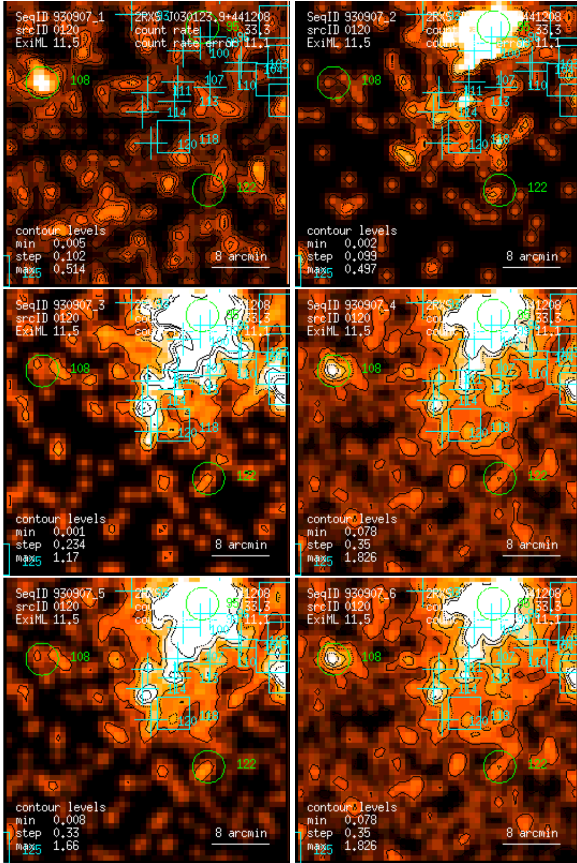
Figure 120: RASS 930907: detection 0120: band rate images, Gaussian filter: (1) PSPC channels 11 – 41, (2) 52 – 90, (3) 91 – 201, (4) 11 – 235, (5) 52 – 201, (6) 11 – 201. Broad band rates in counts/ks. Band rate contour levels in counts/ks/arcmin 2 .
