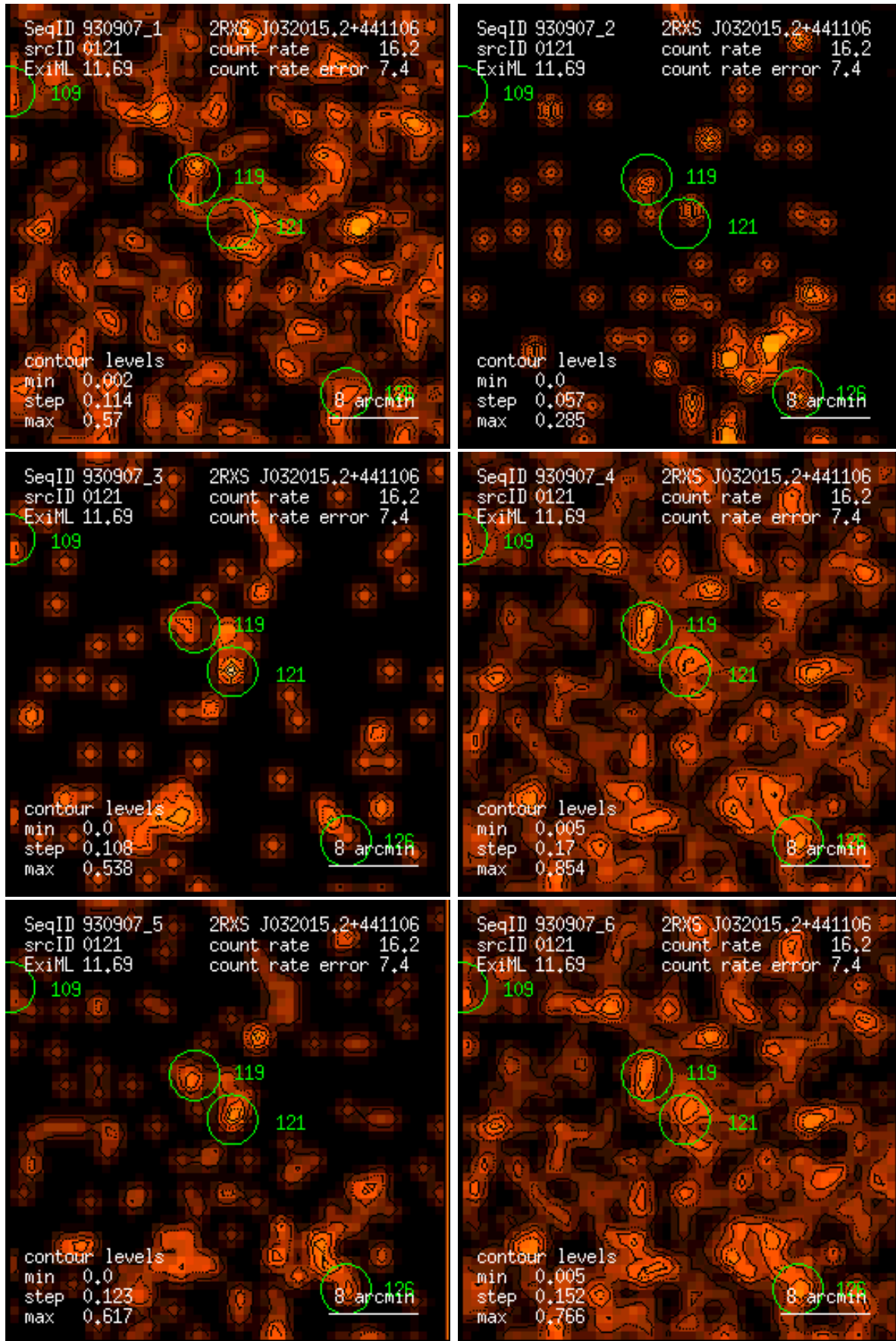
Figure 121: RASS 930907: detection 0121: band rate images, Gaussian filter: (1) PSPC channels 11 – 41, (2) 52 – 90, (3) 91 – 201, (4) 11 – 235, (5) 52 – 201, (6) 11 – 201. Broad band rates in counts/ks. Band rate contour levels in counts/ks/arcmin 2 .
