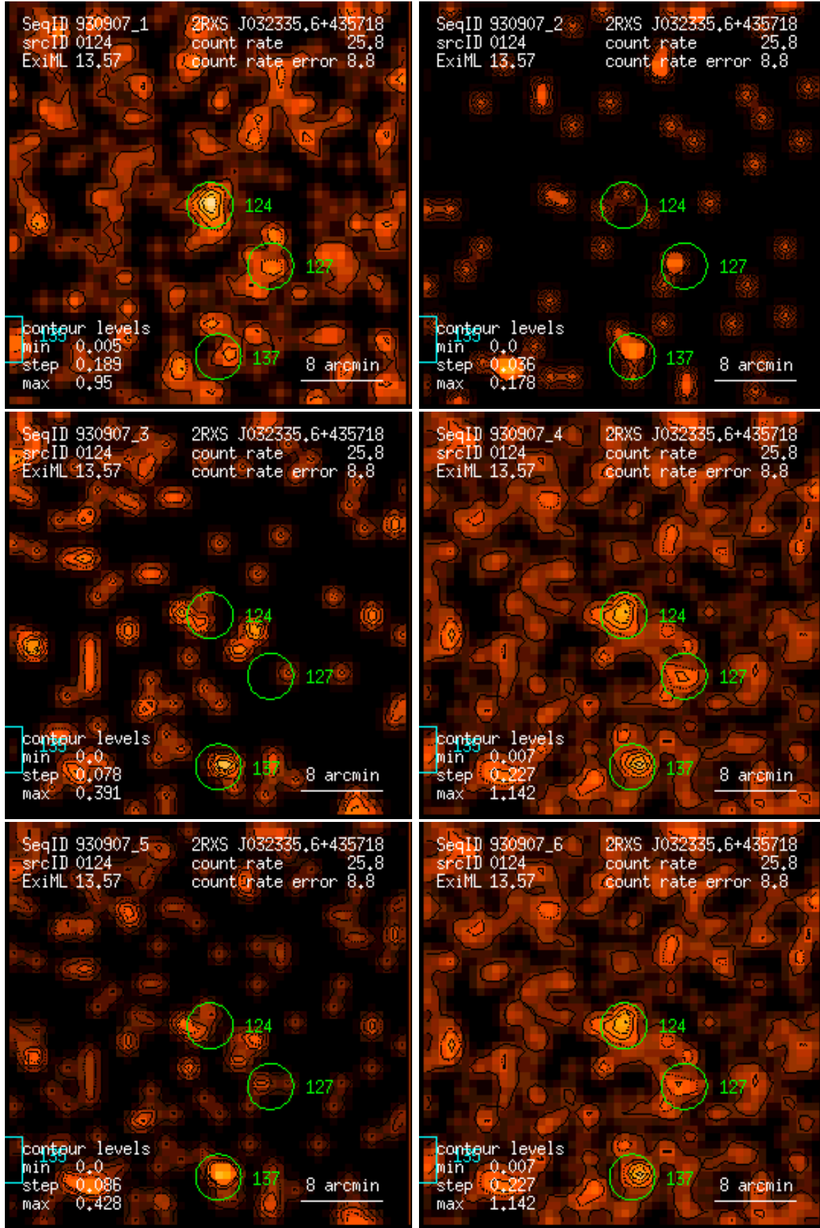
Figure 124: RASS 930907: detection 0124: band rate images, Gaussian filter: (1) PSPC channels 11 – 41, (2) 52 – 90, (3) 91 – 201, (4) 11 – 235, (5) 52 – 201, (6) 11 – 201. Broad band rates in counts/ks. Band rate contour levels in counts/ks/arcmin 2 .
