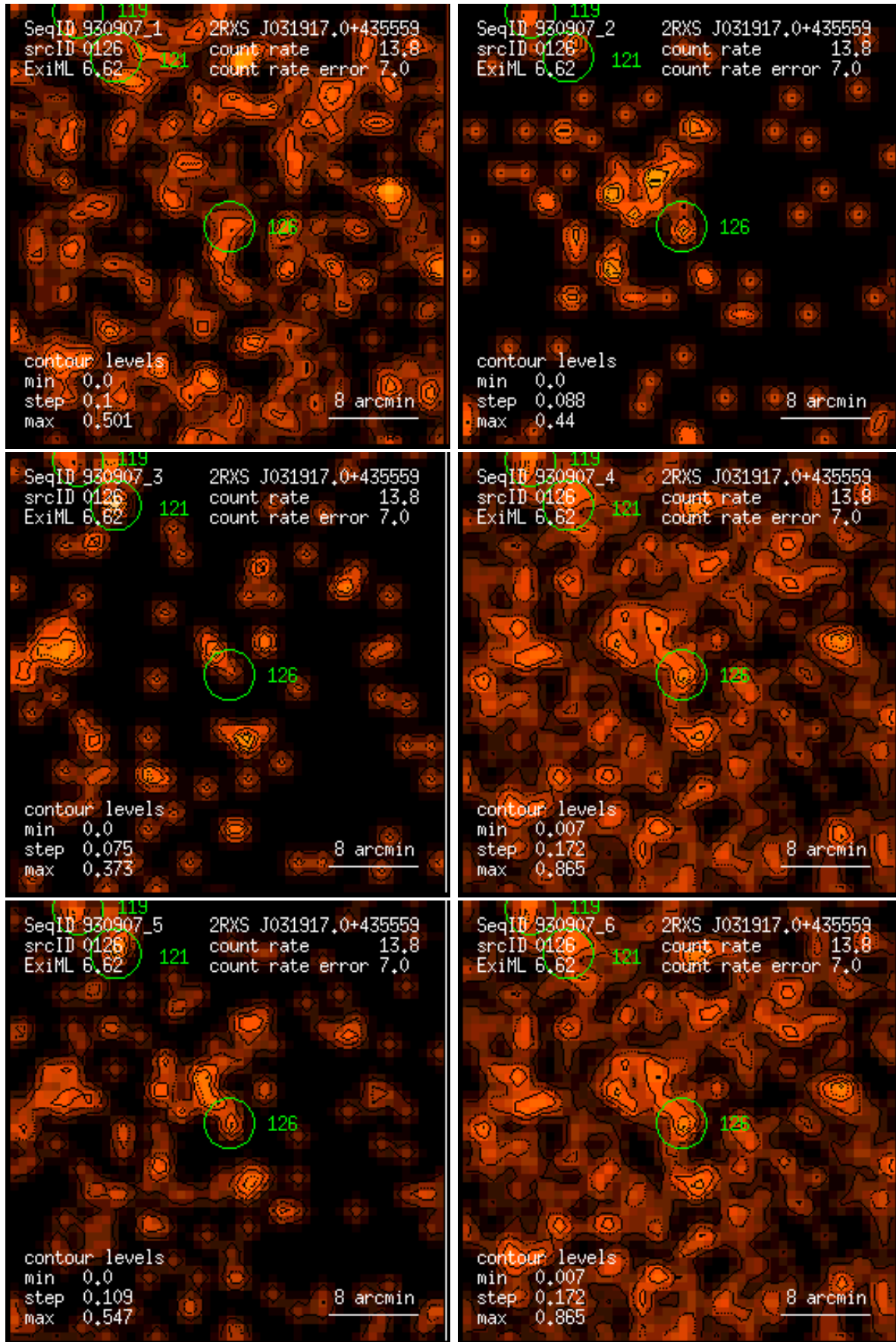
Figure 126: RASS 930907: detection 0126: band rate images, Gaussian filter: (1) PSPC channels 11 – 41, (2) 52 – 90, (3) 91 – 201, (4) 11 – 235, (5) 52 – 201, (6) 11 – 201. Broad band rates in counts/ks. Band rate contour levels in counts/ks/arcmin 2 .
