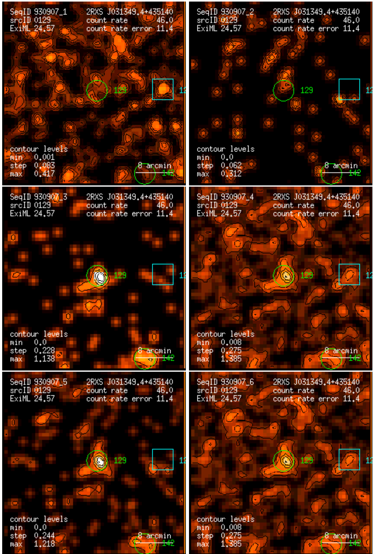
Figure 129: RASS 930907: detection 0129: band rate images, Gaussian filter: (1) PSPC channels 11 – 41, (2) 52 – 90, (3) 91 – 201, (4) 11 – 235, (5) 52 – 201, (6) 11 – 201. Broad band rates in counts/ks. Band rate contour levels in counts/ks/arcmin 2 .
