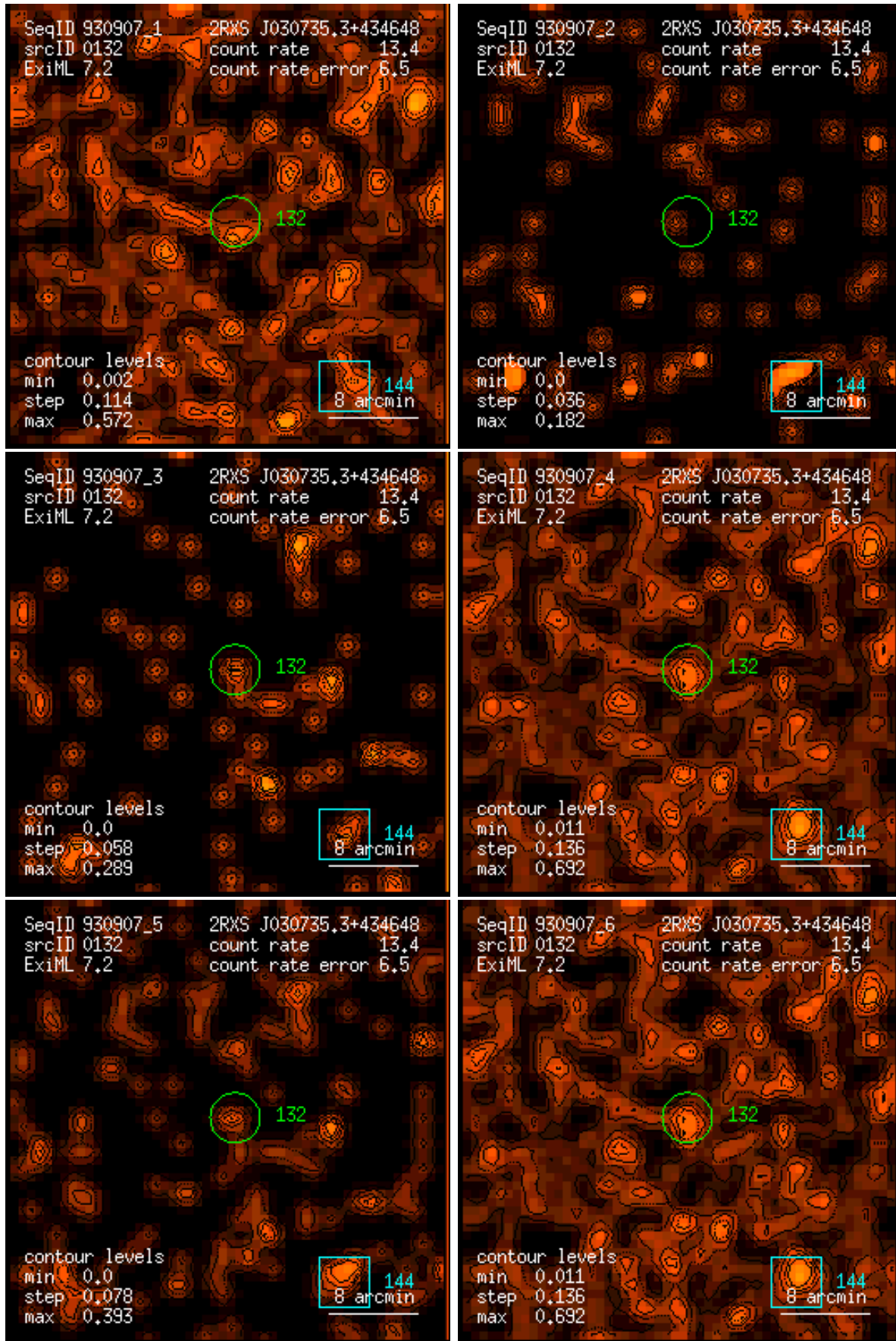
Figure 132: RASS 930907: detection 0132: band rate images, Gaussian filter: (1) PSPC channels 11 – 41, (2) 52 – 90, (3) 91 – 201, (4) 11 – 235, (5) 52 – 201, (6) 11 – 201. Broad band rates in counts/ks. Band rate contour levels in counts/ks/arcmin 2 .
