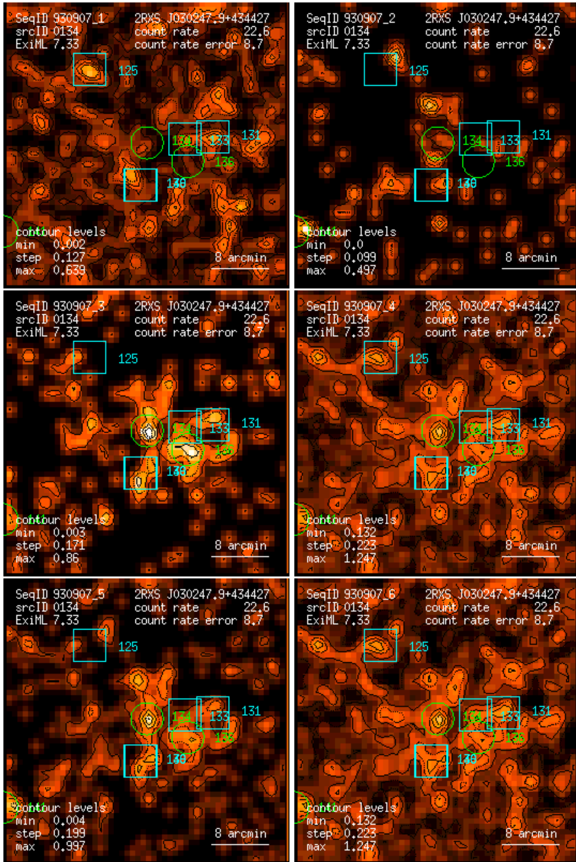
Figure 134: RASS 930907: detection 0134: band rate images, Gaussian filter: (1) PSPC channels 11 – 41, (2) 52 – 90, (3) 91 – 201, (4) 11 – 235, (5) 52 – 201, (6) 11 – 201. Broad band rates in counts/ks. Band rate contour levels in counts/ks/arcmin 2 .
