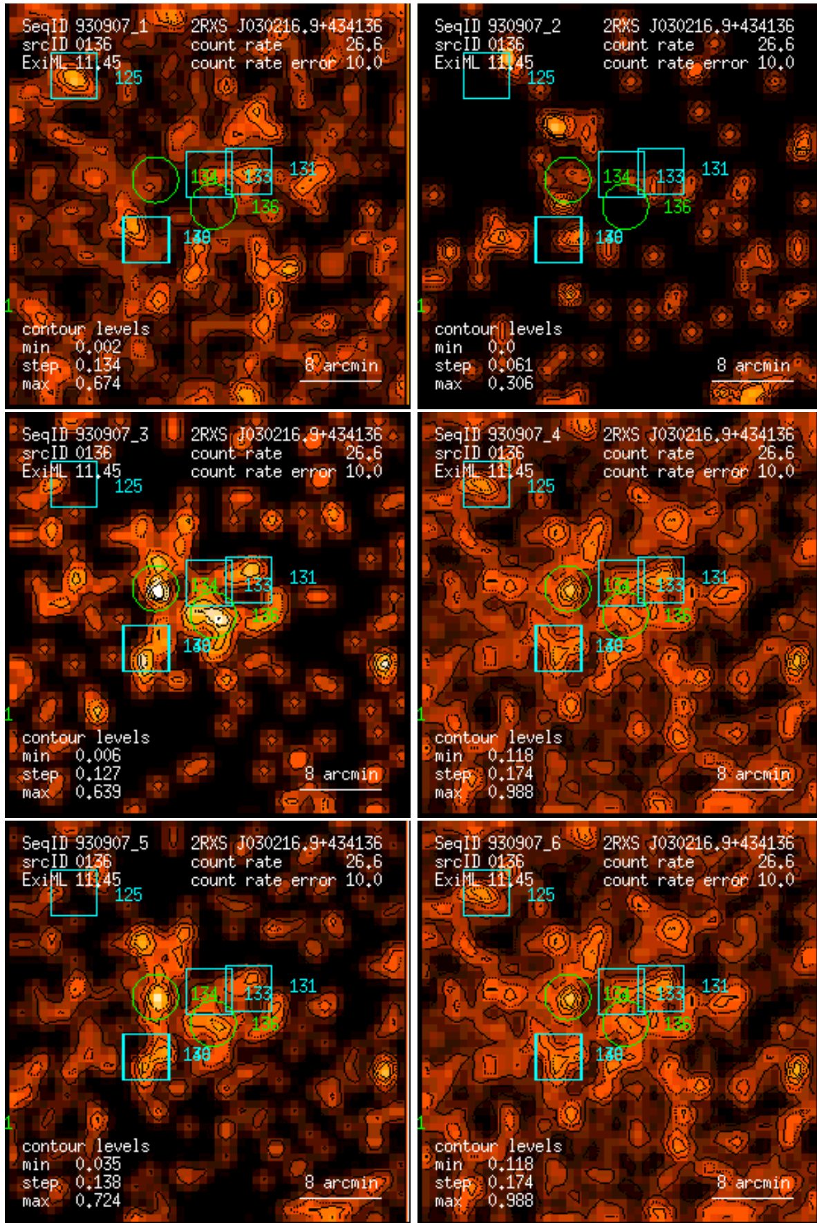
Figure 136: RASS 930907: detection 0136: band rate images, Gaussian filter: (1) PSPC channels 11 – 41, (2) 52 – 90, (3) 91 – 201, (4) 11 – 235, (5) 52 – 201, (6) 11 – 201. Broad band rates in counts/ks. Band rate contour levels in counts/ks/arcmin 2 .
