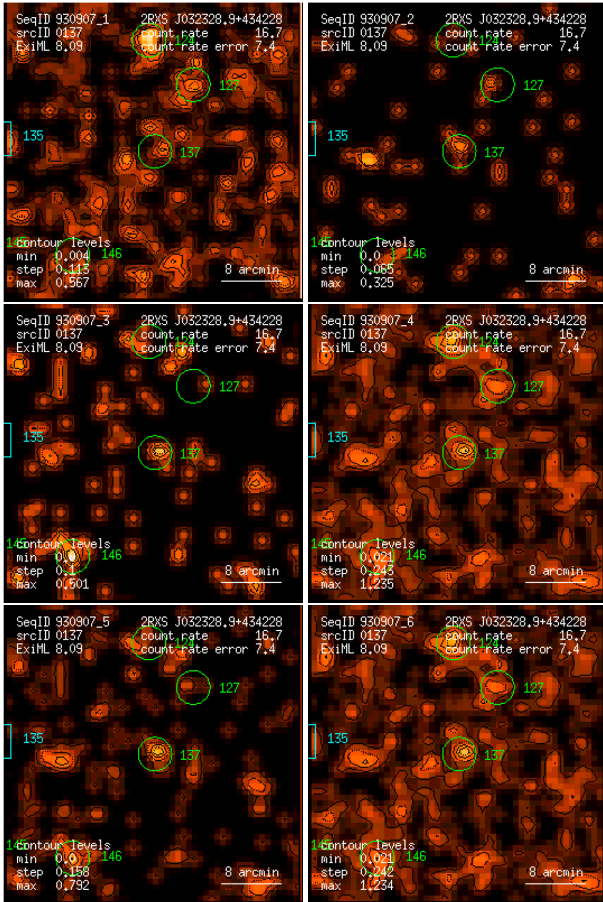
Figure 137: RASS 930907: detection 0137: band rate images, Gaussian filter: (1) PSPC channels 11 – 41, (2) 52 – 90, (3) 91 – 201, (4) 11 – 235, (5) 52 – 201, (6) 11 – 201. Broad band rates in counts/ks. Band rate contour levels in counts/ks/arcmin 2 .
