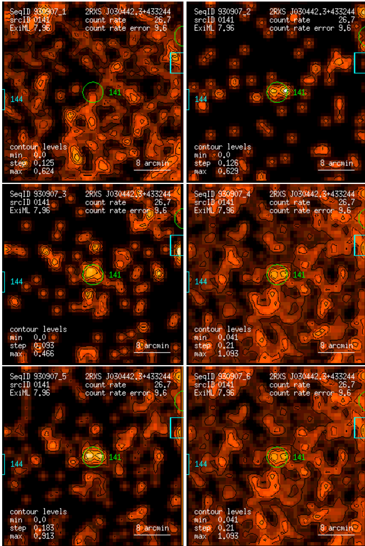
Figure 141: RASS 930907: detection 0141: band rate images, Gaussian filter: (1) PSPC channels 11 – 41, (2) 52 – 90, (3) 91 – 201, (4) 11 – 235, (5) 52 – 201, (6) 11 – 201. Broad band rates in counts/ks. Band rate contour levels in counts/ks/arcmin 2 .
