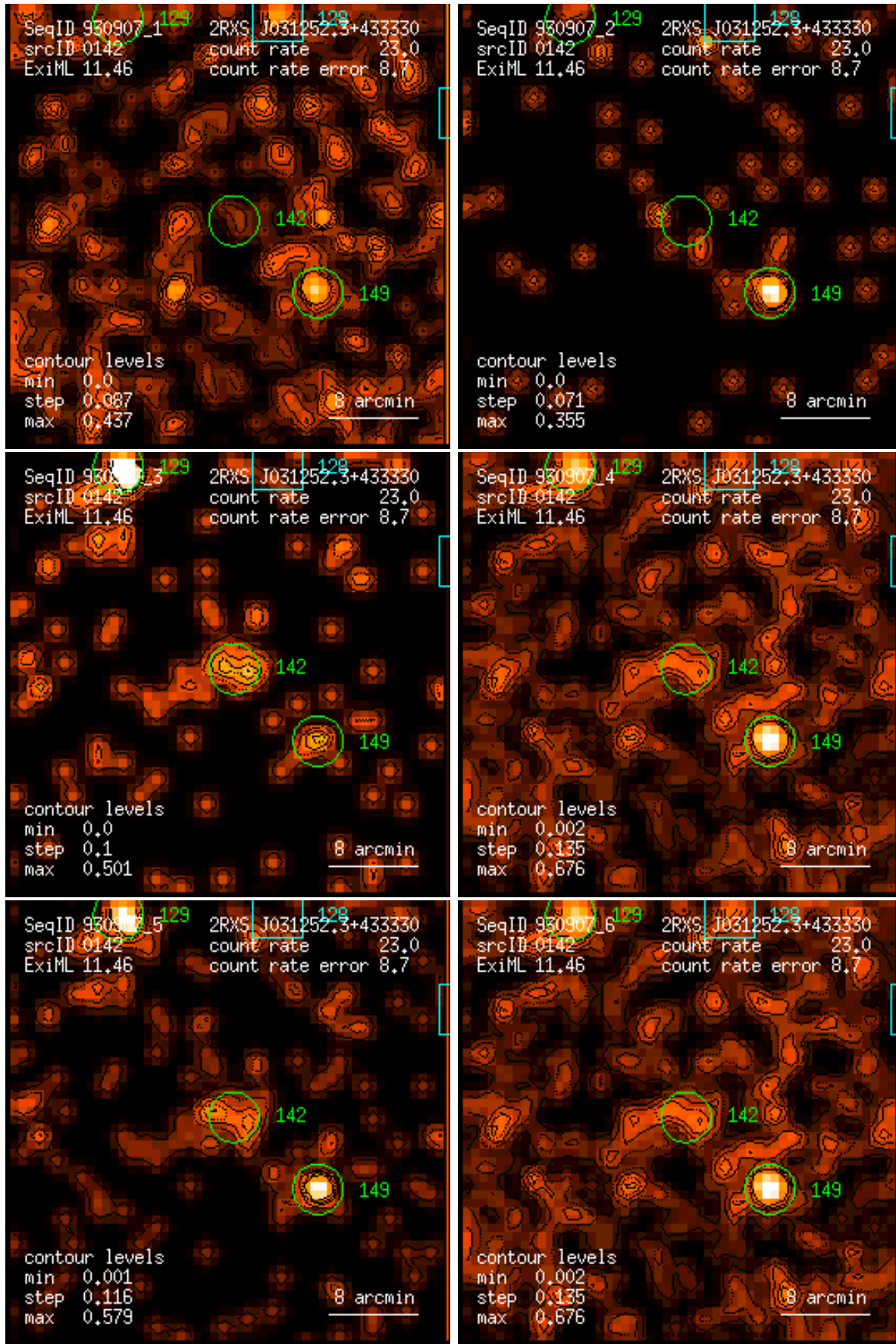
Figure 142: RASS 930907: detection 0142: band rate images, Gaussian filter: (1) PSPC channels 11 – 41, (2) 52 – 90, (3) 91 – 201, (4) 11 – 235, (5) 52 – 201, (6) 11 – 201. Broad band rates in counts/ks. Band rate contour levels in counts/ks/arcmin 2 .
