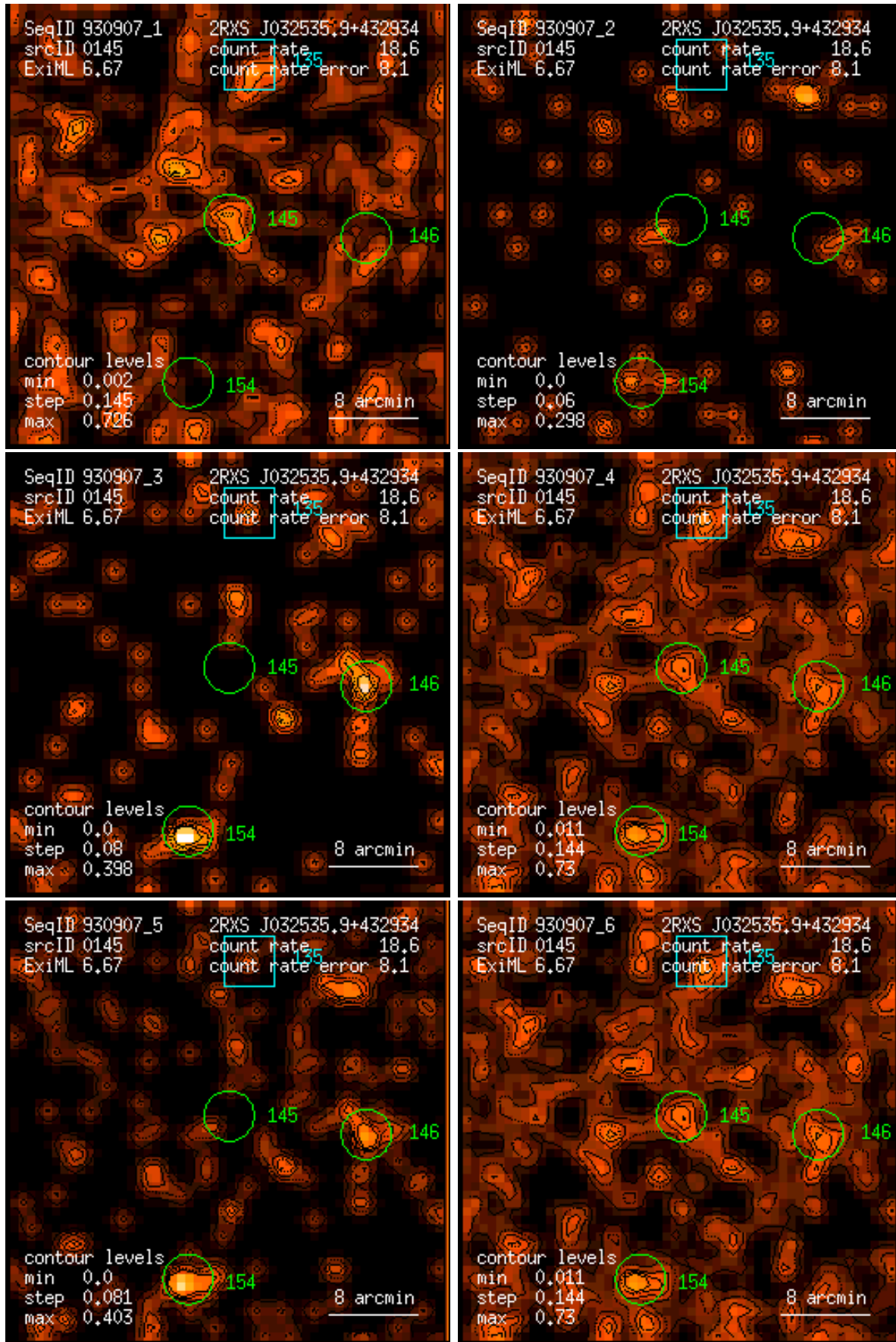
Figure 145: RASS 930907: detection 0145: band rate images, Gaussian filter: (1) PSPC channels 11 – 41, (2) 52 – 90, (3) 91 – 201, (4) 11 – 235, (5) 52 – 201, (6) 11 – 201. Broad band rates in counts/ks. Band rate contour levels in counts/ks/arcmin 2 .
