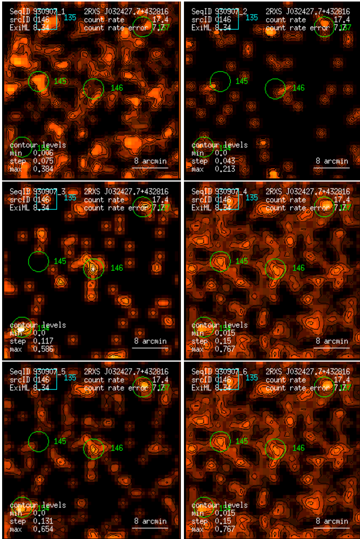
Figure 146: RASS 930907: detection 0146: band rate images, Gaussian filter: (1) PSPC channels 11 – 41, (2) 52 – 90, (3) 91 – 201, (4) 11 – 235, (5) 52 – 201, (6) 11 – 201. Broad band rates in counts/ks. Band rate contour levels in counts/ks/arcmin 2 .
