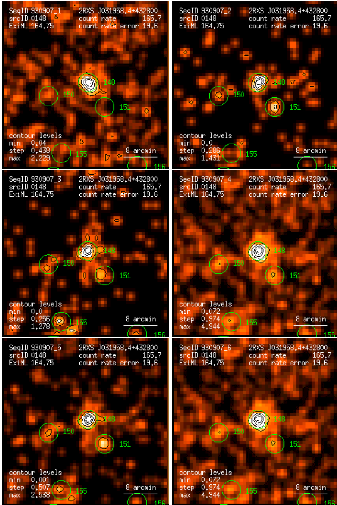
Figure 148: RASS 930907: detection 0148: band rate images, Gaussian filter: (1) PSPC channels 11 – 41, (2) 52 – 90, (3) 91 – 201, (4) 11 – 235, (5) 52 – 201, (6) 11 – 201. Broad band rates in counts/ks. Band rate contour levels in counts/ks/arcmin 2 .
