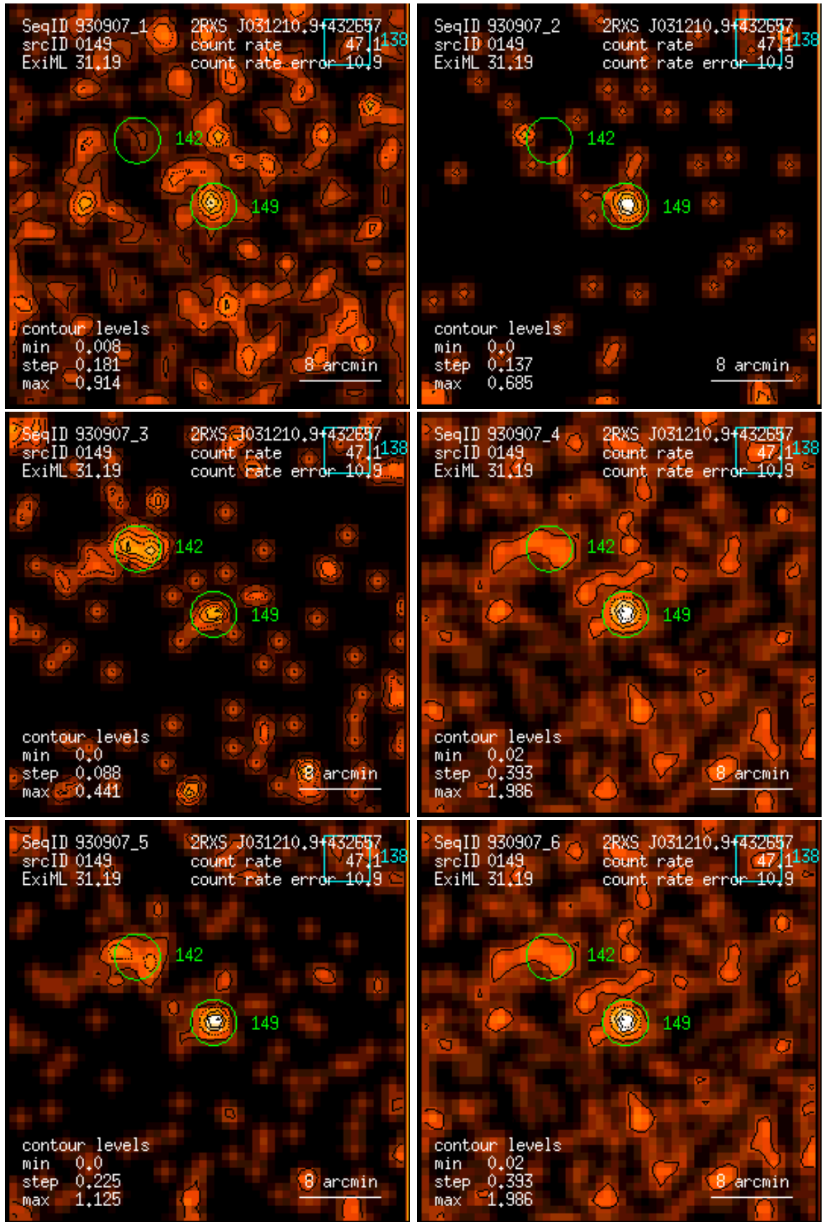
Figure 149: RASS 930907: detection 0149: band rate images, Gaussian filter: (1) PSPC channels 11 – 41, (2) 52 – 90, (3) 91 – 201, (4) 11 – 235, (5) 52 – 201, (6) 11 – 201. Broad band rates in counts/ks. Band rate contour levels in counts/ks/arcmin 2 .
