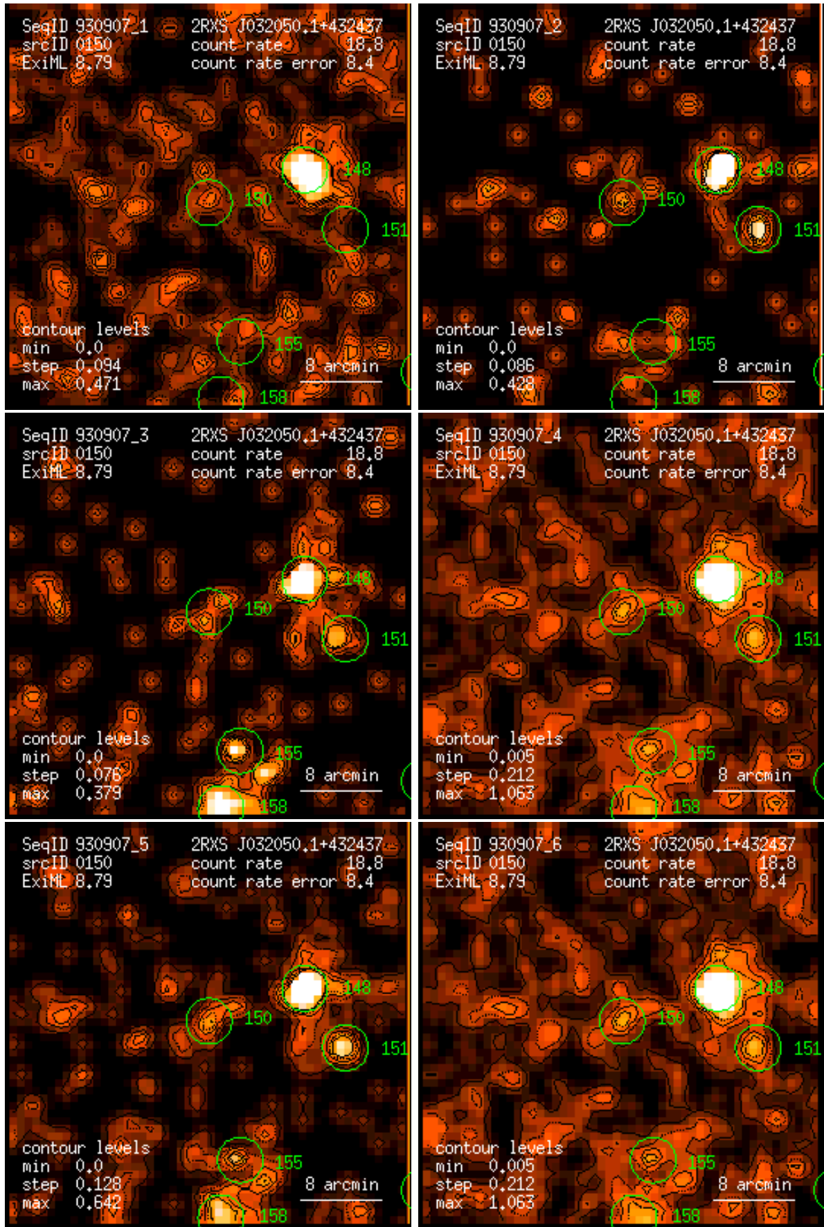
Figure 150: RASS 930907: detection 0150: band rate images, Gaussian filter: (1) PSPC channels 11 – 41, (2) 52 – 90, (3) 91 – 201, (4) 11 – 235, (5) 52 – 201, (6) 11 – 201. Broad band rates in counts/ks. Band rate contour levels in counts/ks/arcmin 2 .
