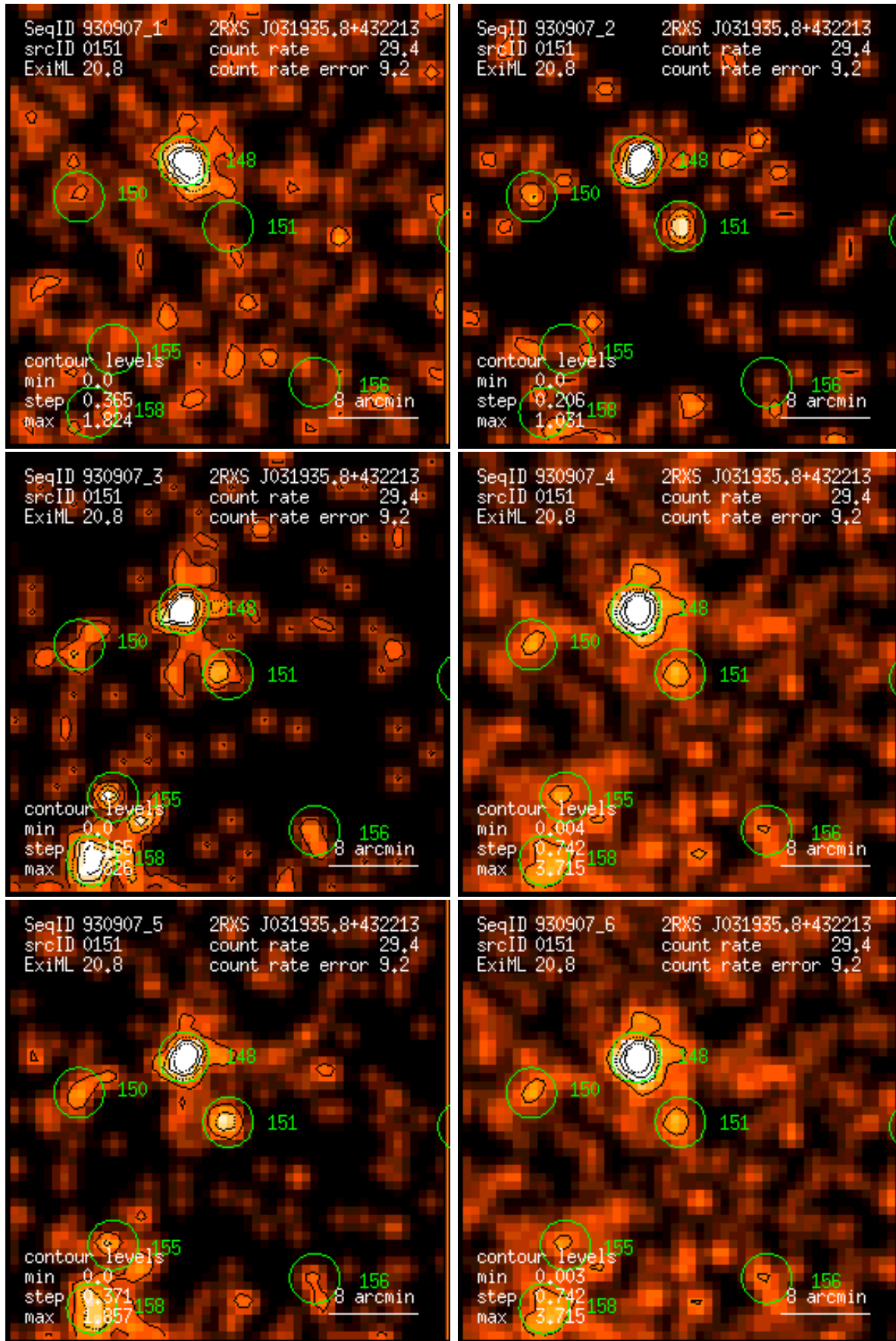
Figure 151: RASS 930907: detection 0151: band rate images, Gaussian filter: (1) PSPC channels 11 – 41, (2) 52 – 90, (3) 91 – 201, (4) 11 – 235, (5) 52 – 201, (6) 11 – 201. Broad band rates in counts/ks. Band rate contour levels in counts/ks/arcmin 2 .
