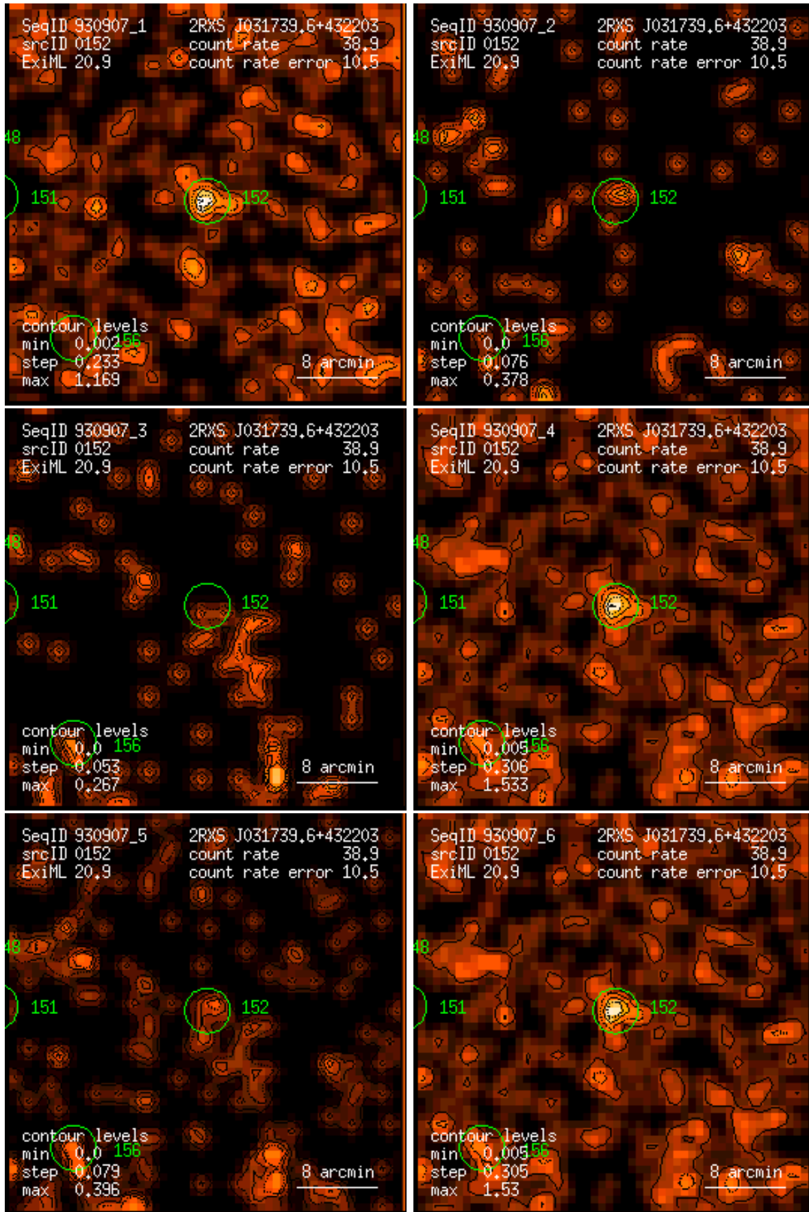
Figure 152: RASS 930907: detection 0152: band rate images, Gaussian filter: (1) PSPC channels 11 – 41, (2) 52 – 90, (3) 91 – 201, (4) 11 – 235, (5) 52 – 201, (6) 11 – 201. Broad band rates in counts/ks. Band rate contour levels in counts/ks/arcmin 2 .
