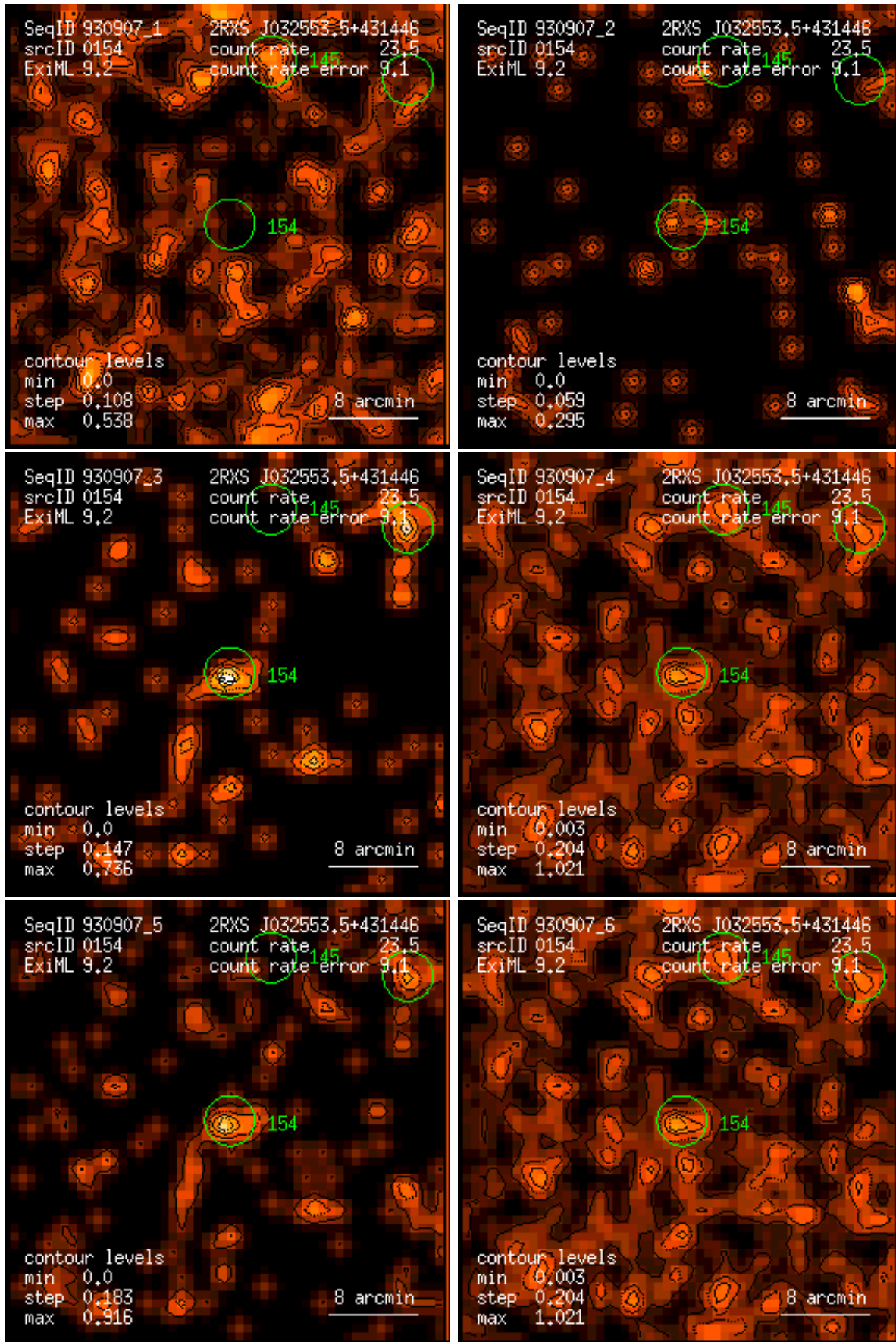
Figure 154: RASS 930907: detection 0154: band rate images, Gaussian filter: (1) PSPC channels 11 – 41, (2) 52 – 90, (3) 91 – 201, (4) 11 – 235, (5) 52 – 201, (6) 11 – 201. Broad band rates in counts/ks. Band rate contour levels in counts/ks/arcmin 2 .
