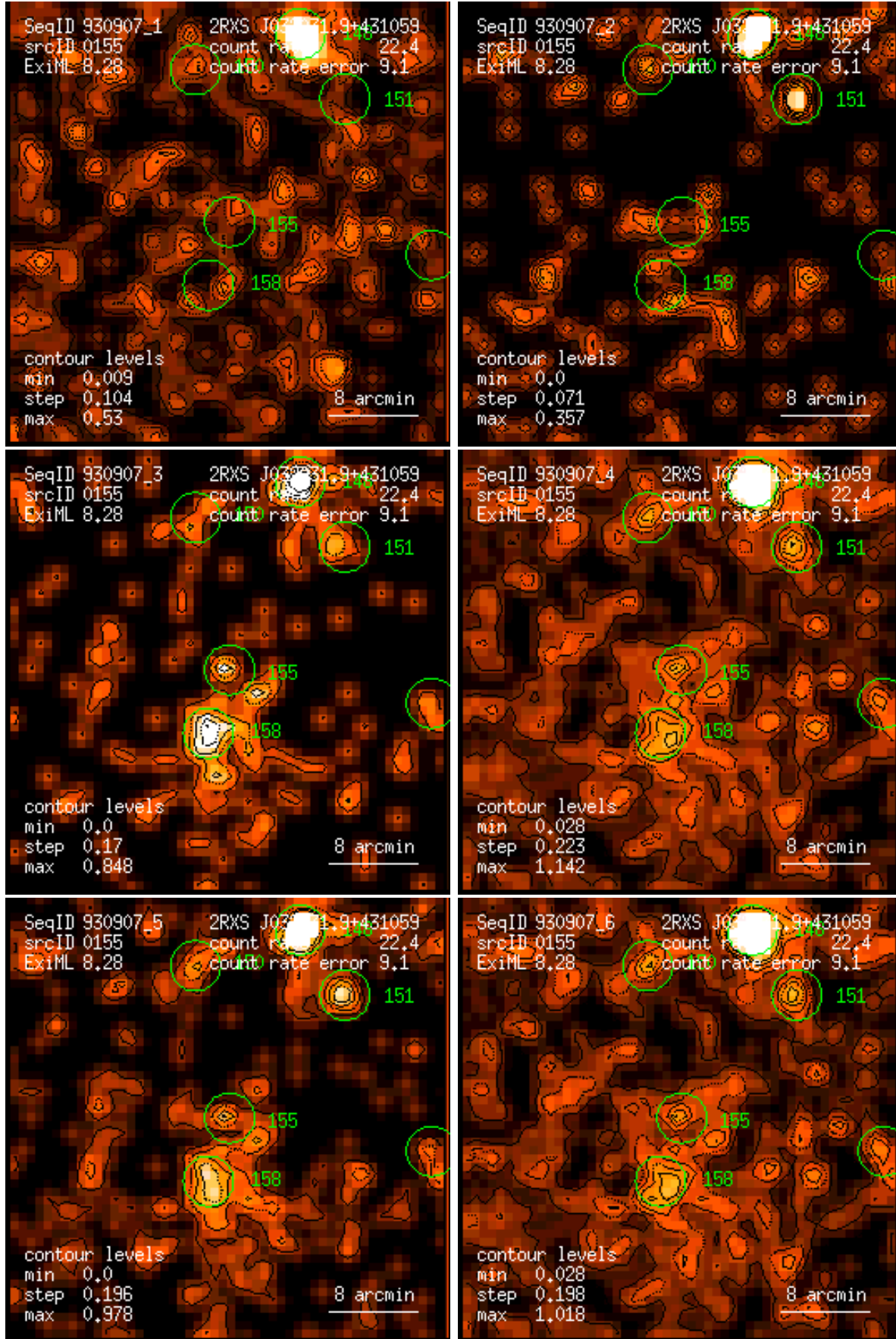
Figure 155: RASS 930907: detection 0155: band rate images, Gaussian filter: (1) PSPC channels 11 – 41, (2) 52 – 90, (3) 91 – 201, (4) 11 – 235, (5) 52 – 201, (6) 11 – 201. Broad band rates in counts/ks. Band rate contour levels in counts/ks/arcmin 2 .
