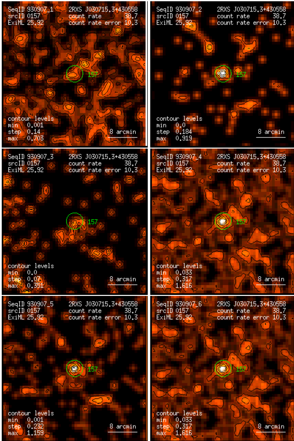
Figure 157: RASS 930907: detection 0157: band rate images, Gaussian filter: (1) PSPC channels 11 – 41, (2) 52 – 90, (3) 91 – 201, (4) 11 – 235, (5) 52 – 201, (6) 11 – 201. Broad band rates in counts/ks. Band rate contour levels in counts/ks/arcmin 2 .
