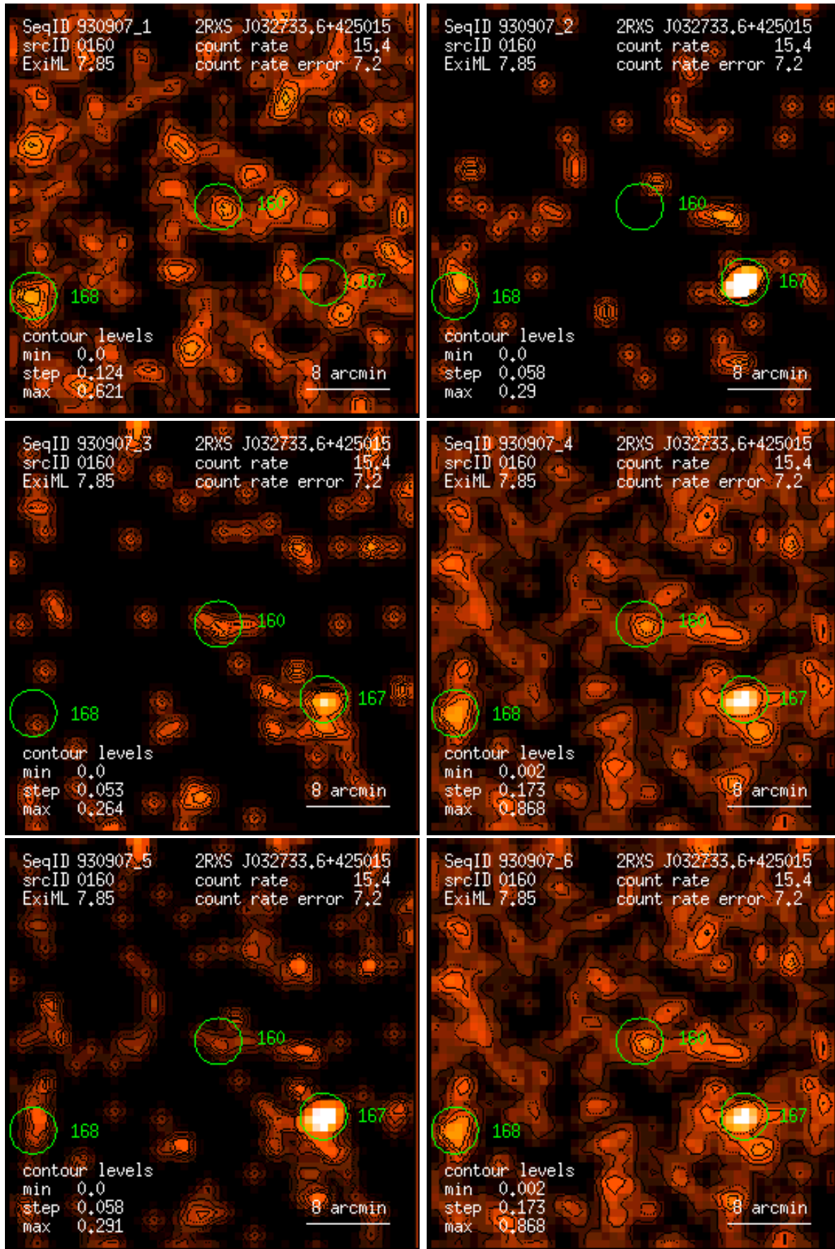
Figure 160: RASS 930907: detection 0160: band rate images, Gaussian filter: (1) PSPC channels 11 – 41, (2) 52 – 90, (3) 91 – 201, (4) 11 – 235, (5) 52 – 201, (6) 11 – 201. Broad band rates in counts/ks. Band rate contour levels in counts/ks/arcmin 2 .
