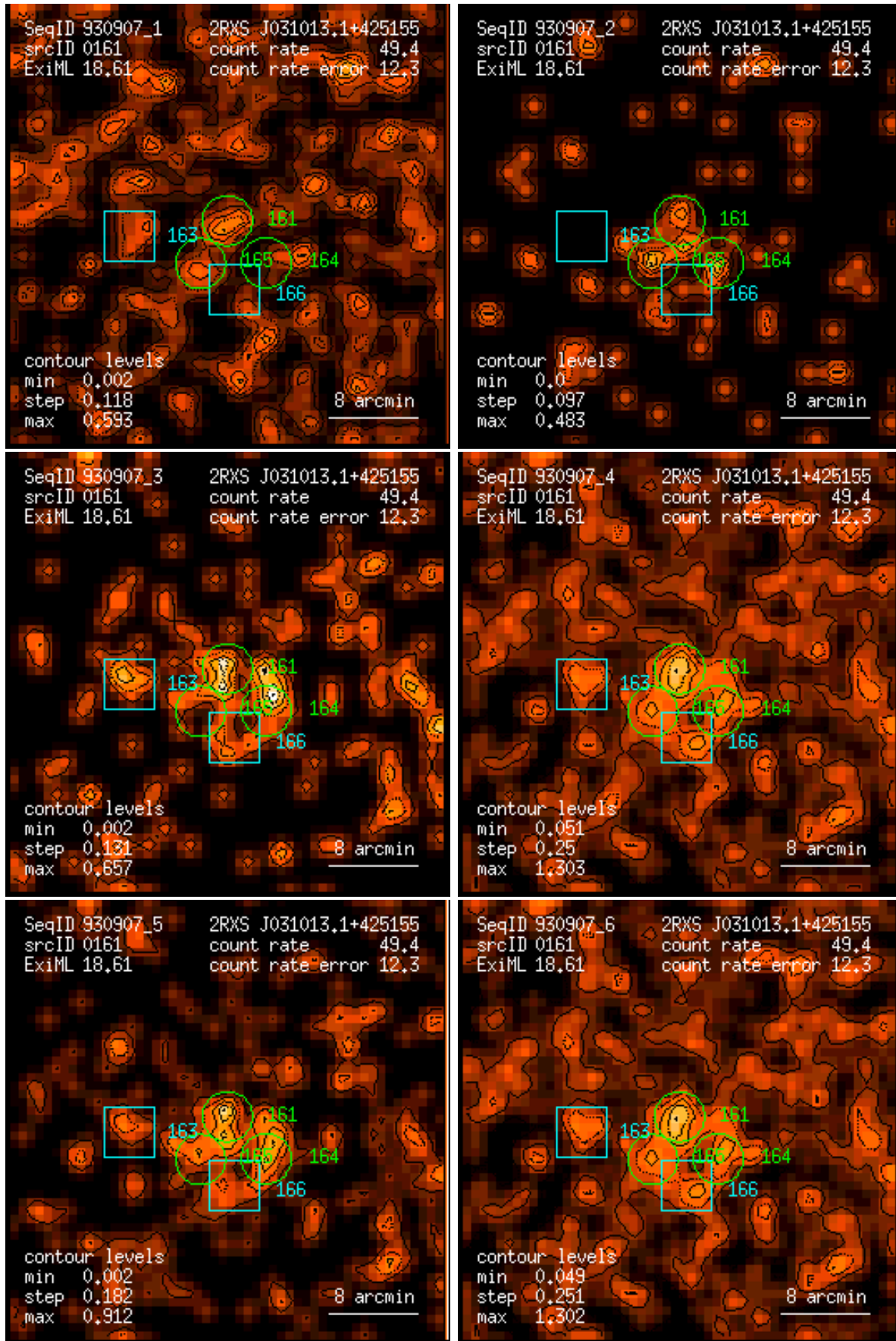
Figure 161: RASS 930907: detection 0161: band rate images, Gaussian filter: (1) PSPC channels 11 – 41, (2) 52 – 90, (3) 91 – 201, (4) 11 – 235, (5) 52 – 201, (6) 11 – 201. Broad band rates in counts/ks. Band rate contour levels in counts/ks/arcmin 2 .
