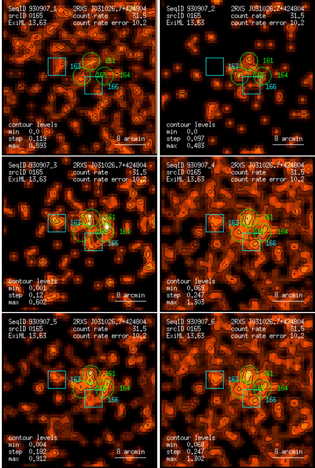
Figure 165: RASS 930907: detection 0165: band rate images, Gaussian filter: (1) PSPC channels 11 – 41, (2) 52 – 90, (3) 91 – 201, (4) 11 – 235, (5) 52 – 201, (6) 11 – 201. Broad band rates in counts/ks. Band rate contour levels in counts/ks/arcmin 2 .
