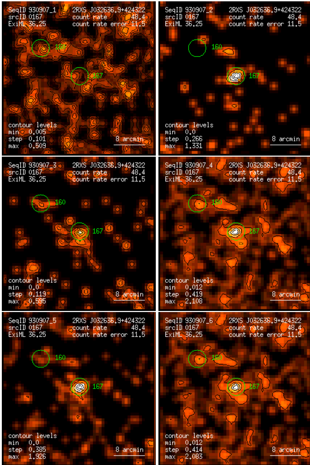
Figure 167: RASS 930907: detection 0167: band rate images, Gaussian filter: (1) PSPC channels 11 – 41, (2) 52 – 90, (3) 91 – 201, (4) 11 – 235, (5) 52 – 201, (6) 11 – 201. Broad band rates in counts/ks. Band rate contour levels in counts/ks/arcmin 2 .
