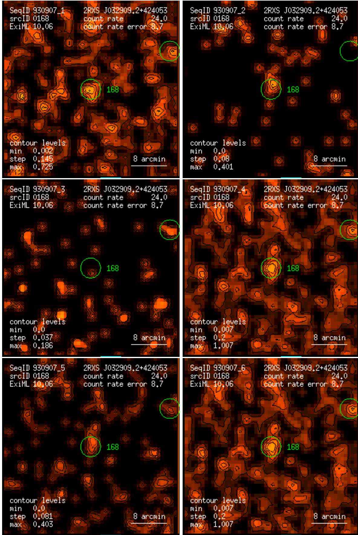
Figure 168: RASS 930907: detection 0168: band rate images, Gaussian filter: (1) PSPC channels 11 – 41, (2) 52 – 90, (3) 91 – 201, (4) 11 – 235, (5) 52 – 201, (6) 11 – 201. Broad band rates in counts/ks. Band rate contour levels in counts/ks/arcmin 2 .
