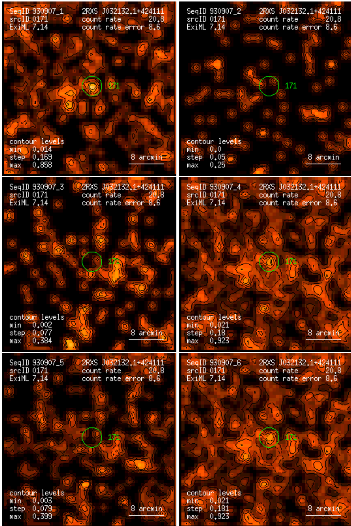
Figure 171: RASS 930907: detection 0171: band rate images, Gaussian filter: (1) PSPC channels 11 – 41, (2) 52 – 90, (3) 91 – 201, (4) 11 – 235, (5) 52 – 201, (6) 11 – 201. Broad band rates in counts/ks. Band rate contour levels in counts/ks/arcmin 2 .
