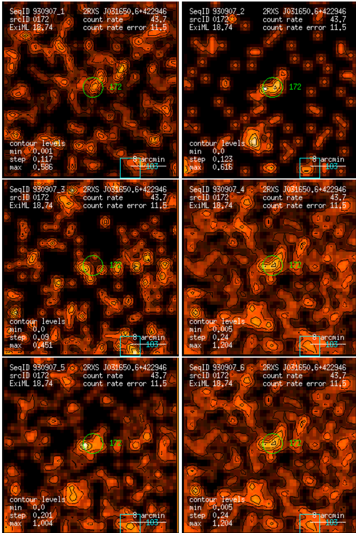
Figure 172: RASS 930907: detection 0172: band rate images, Gaussian filter: (1) PSPC channels 11 – 41, (2) 52 – 90, (3) 91 – 201, (4) 11 – 235, (5) 52 – 201, (6) 11 – 201. Broad band rates in counts/ks. Band rate contour levels in counts/ks/arcmin 2 .
