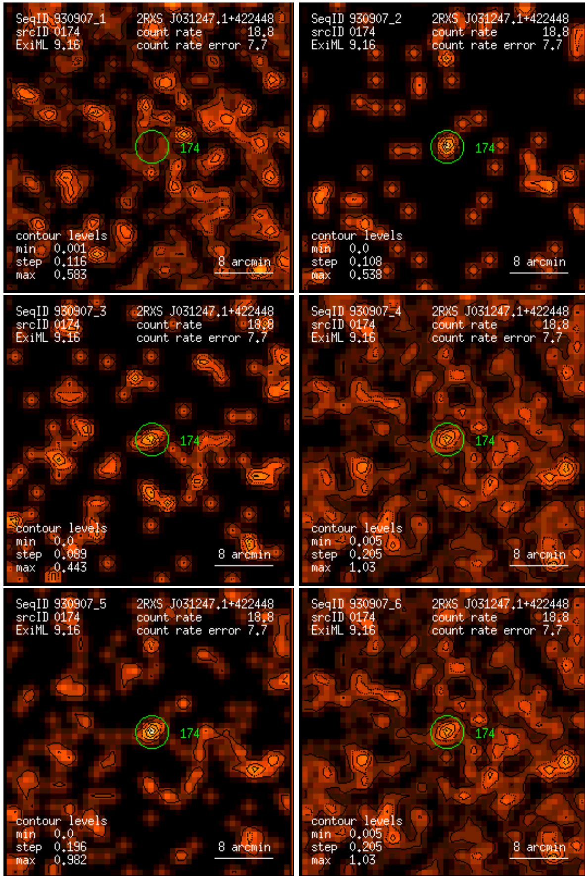
Figure 174: RASS 930907: detection 0174: band rate images, Gaussian filter: (1) PSPC channels 11 – 41, (2) 52 – 90, (3) 91 – 201, (4) 11 – 235, (5) 52 – 201, (6) 11 – 201. Broad band rates in counts/ks. Band rate contour levels in counts/ks/arcmin 2 .
