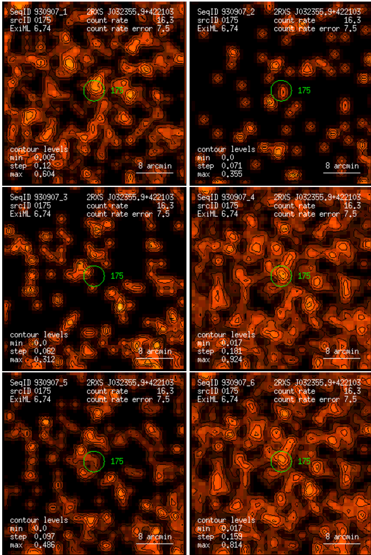
Figure 175: RASS 930907: detection 0175: band rate images, Gaussian filter: (1) PSPC channels 11 – 41, (2) 52 – 90, (3) 91 – 201, (4) 11 – 235, (5) 52 – 201, (6) 11 – 201. Broad band rates in counts/ks. Band rate contour levels in counts/ks/arcmin 2 .
