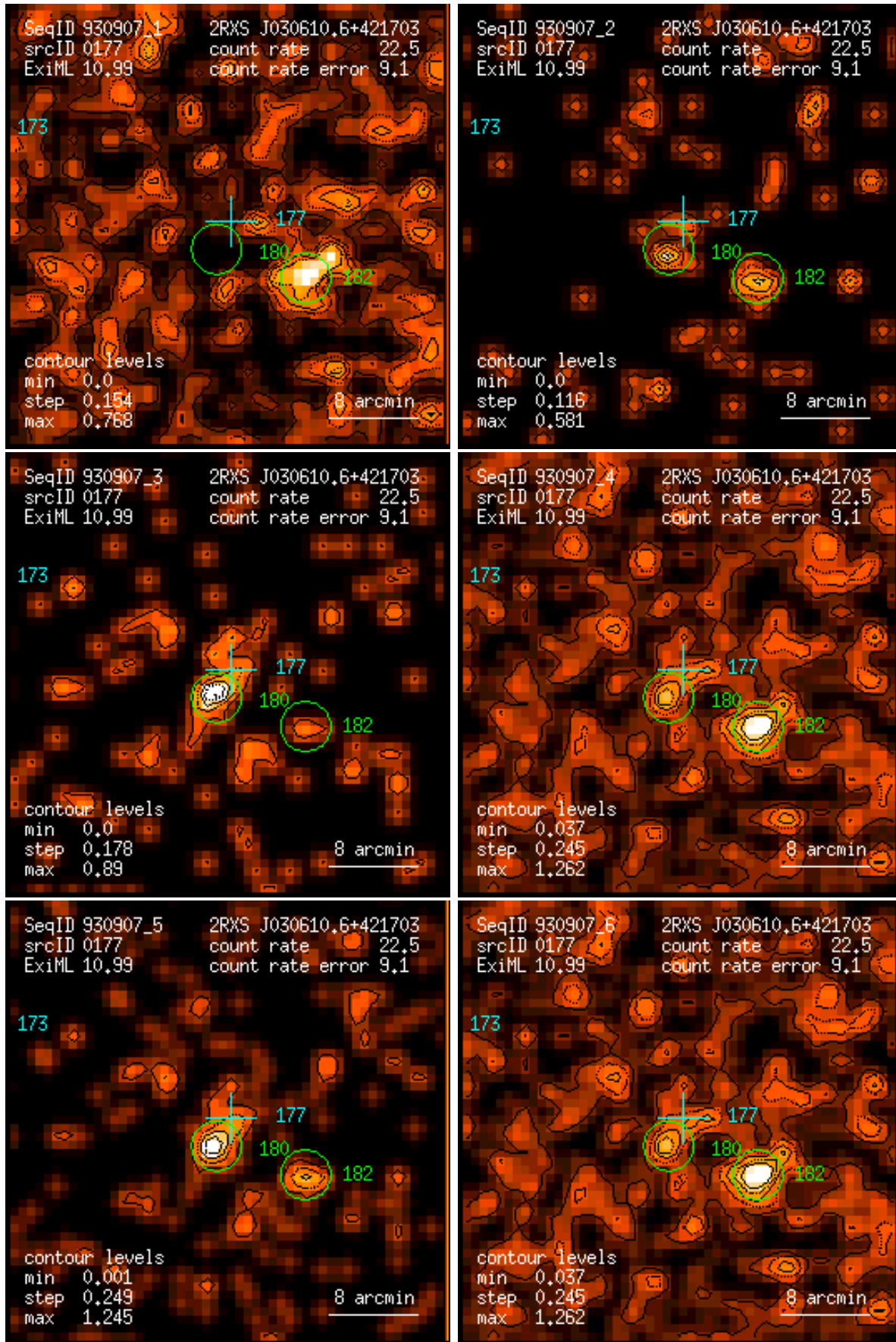
Figure 177: RASS 930907: detection 0177: band rate images, Gaussian filter: (1) PSPC channels 11 – 41, (2) 52 – 90, (3) 91 – 201, (4) 11 – 235, (5) 52 – 201, (6) 11 – 201. Broad band rates in counts/ks. Band rate contour levels in counts/ks/arcmin 2 .
