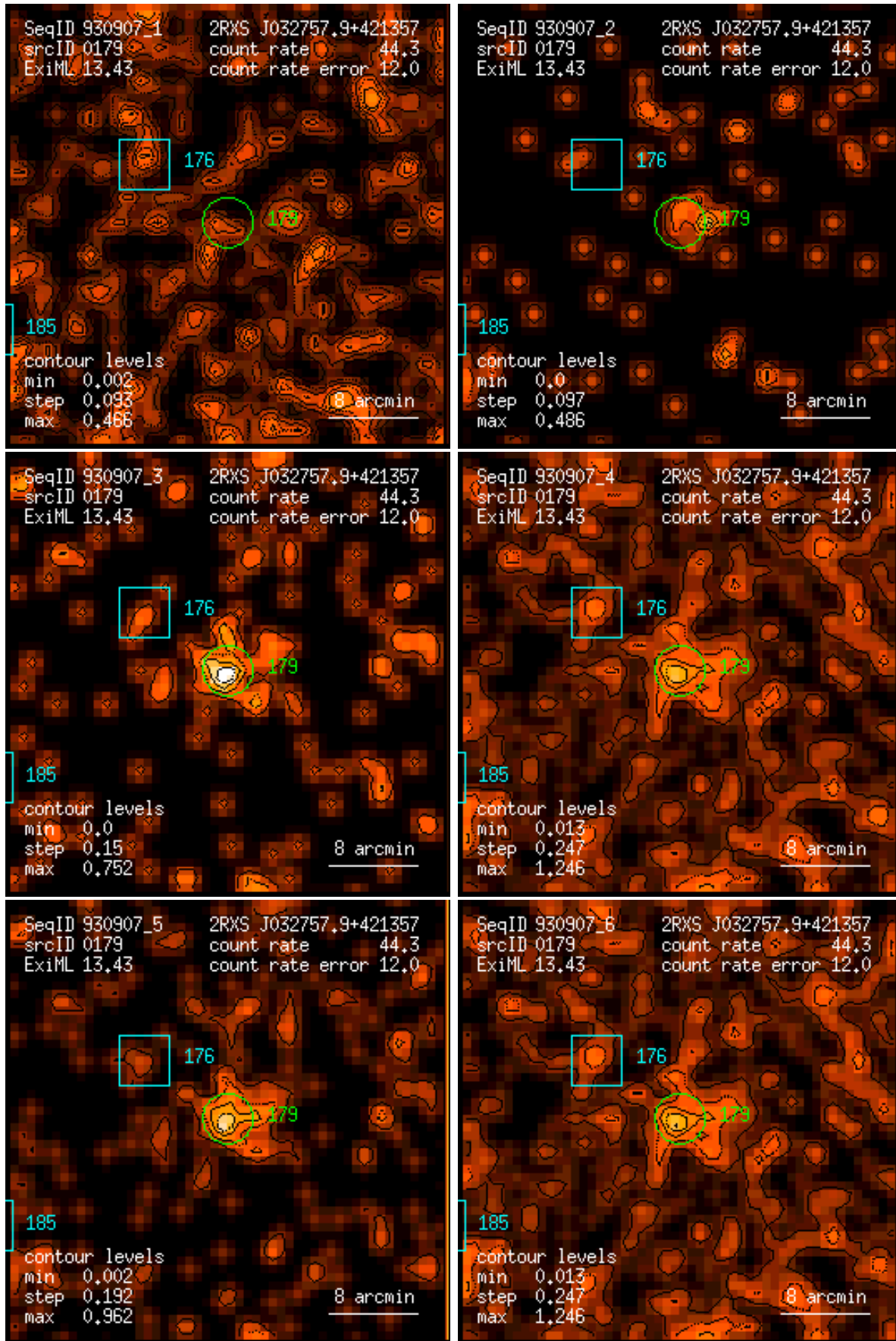
Figure 179: RASS 930907: detection 0179: band rate images, Gaussian filter: (1) PSPC channels 11 – 41, (2) 52 – 90, (3) 91 – 201, (4) 11 – 235, (5) 52 – 201, (6) 11 – 201. Broad band rates in counts/ks. Band rate contour levels in counts/ks/arcmin 2 .
