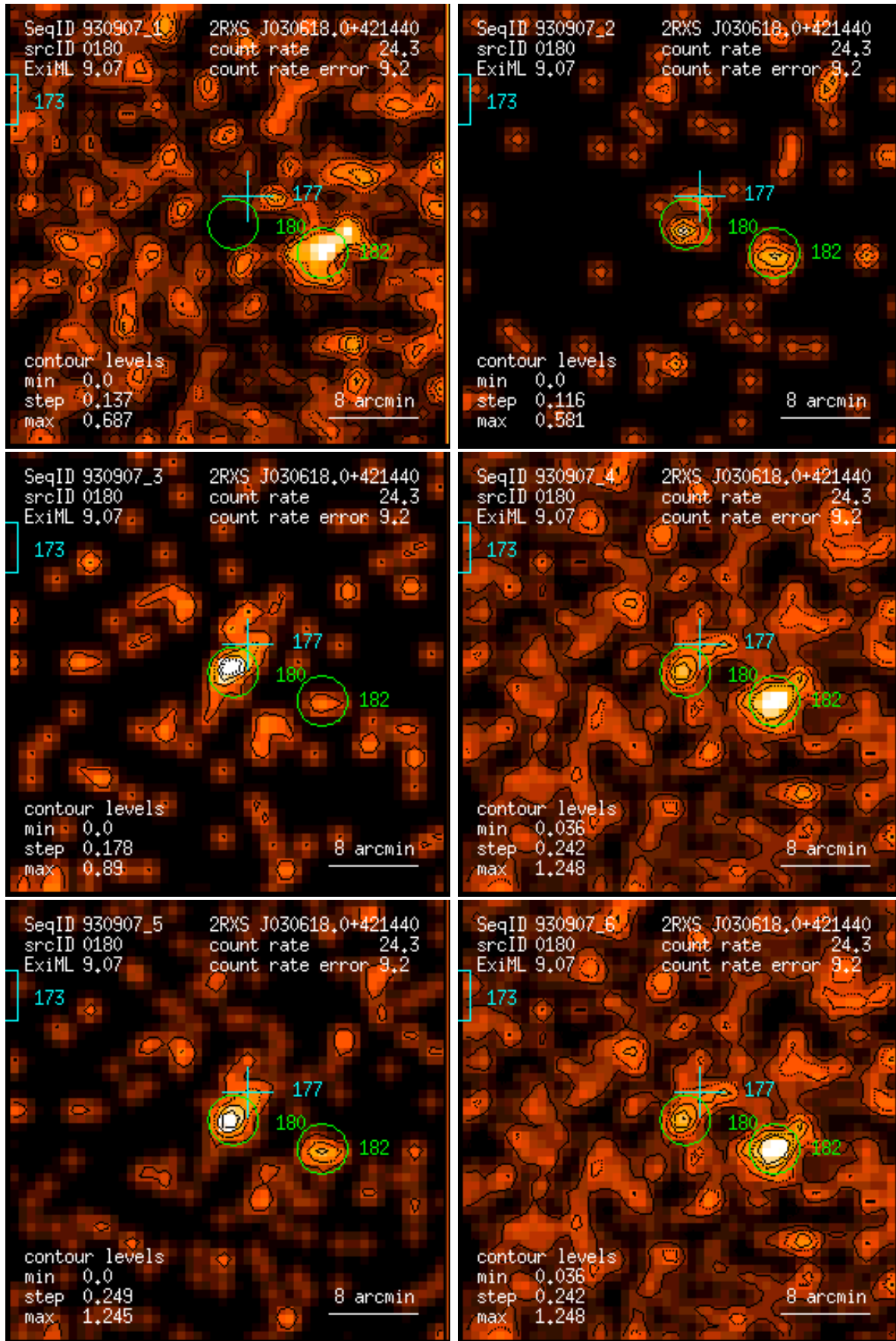
Figure 180: RASS 930907: detection 0180: band rate images, Gaussian filter: (1) PSPC channels 11 – 41, (2) 52 – 90, (3) 91 – 201, (4) 11 – 235, (5) 52 – 201, (6) 11 – 201. Broad band rates in counts/ks. Band rate contour levels in counts/ks/arcmin 2 .
