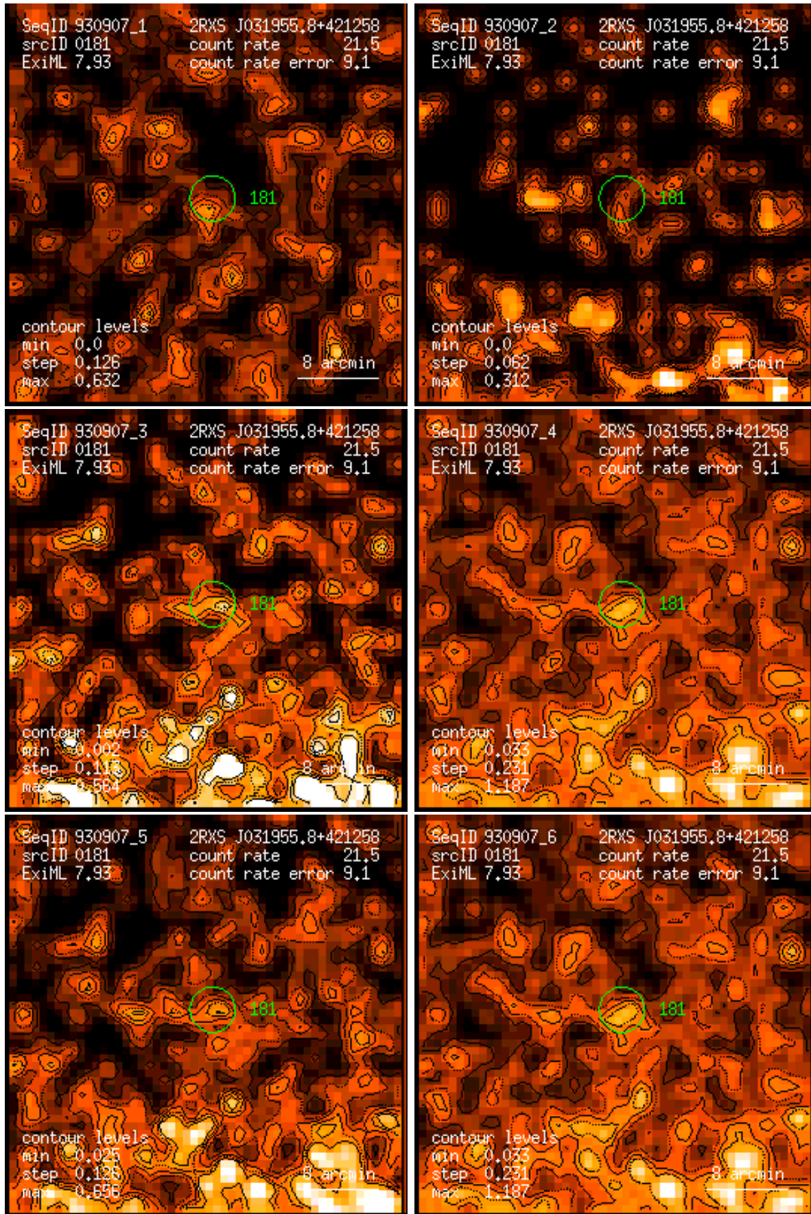
Figure 181: RASS 930907: detection 0181: band rate images, Gaussian filter: (1) PSPC channels 11 – 41, (2) 52 – 90, (3) 91 – 201, (4) 11 – 235, (5) 52 – 201, (6) 11 – 201. Broad band rates in counts/ks. Band rate contour levels in counts/ks/arcmin 2 .
