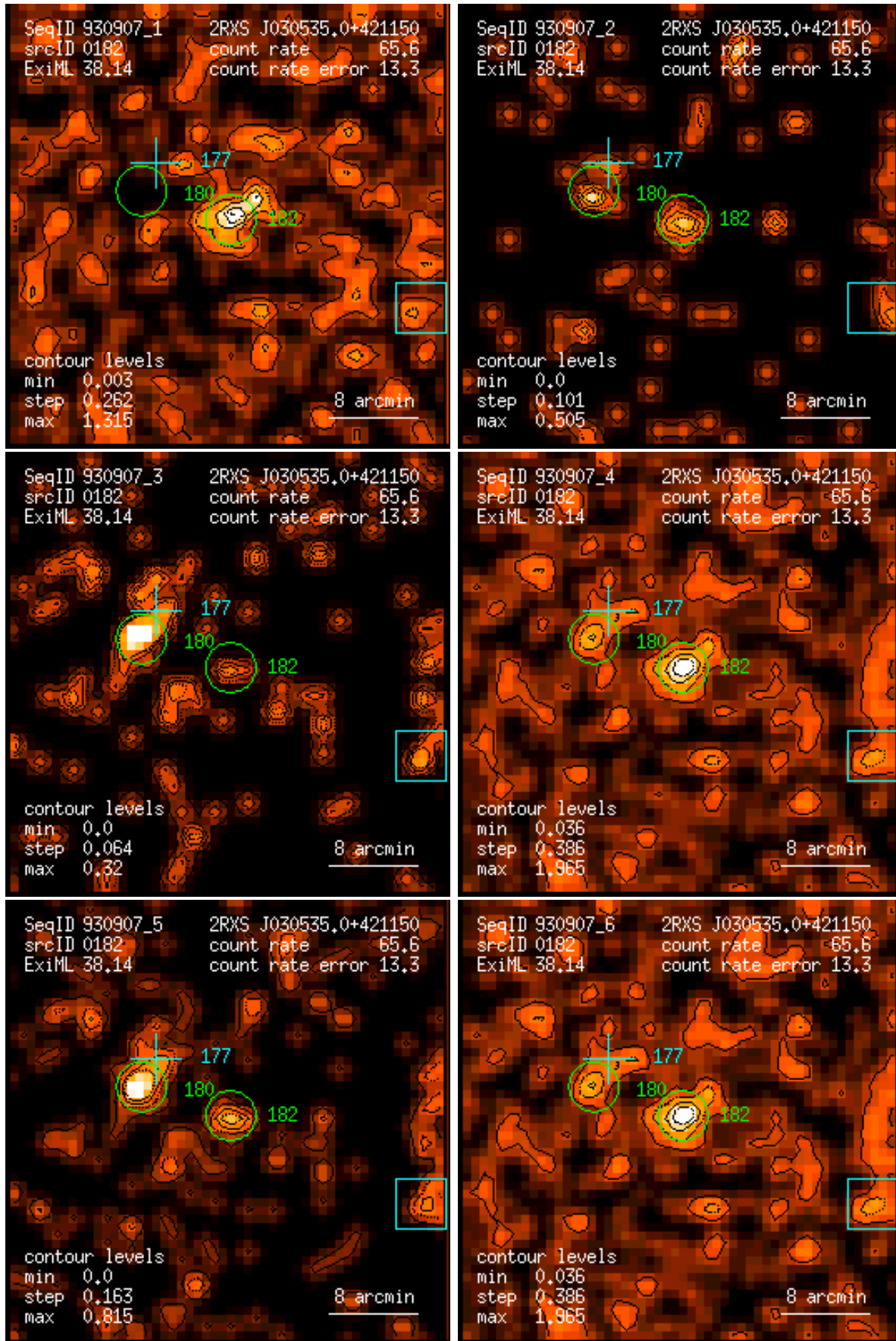
Figure 182: RASS 930907: detection 0182: band rate images, Gaussian filter: (1) PSPC channels 11 – 41, (2) 52 – 90, (3) 91 – 201, (4) 11 – 235, (5) 52 – 201, (6) 11 – 201. Broad band rates in counts/ks. Band rate contour levels in counts/ks/arcmin 2 .
