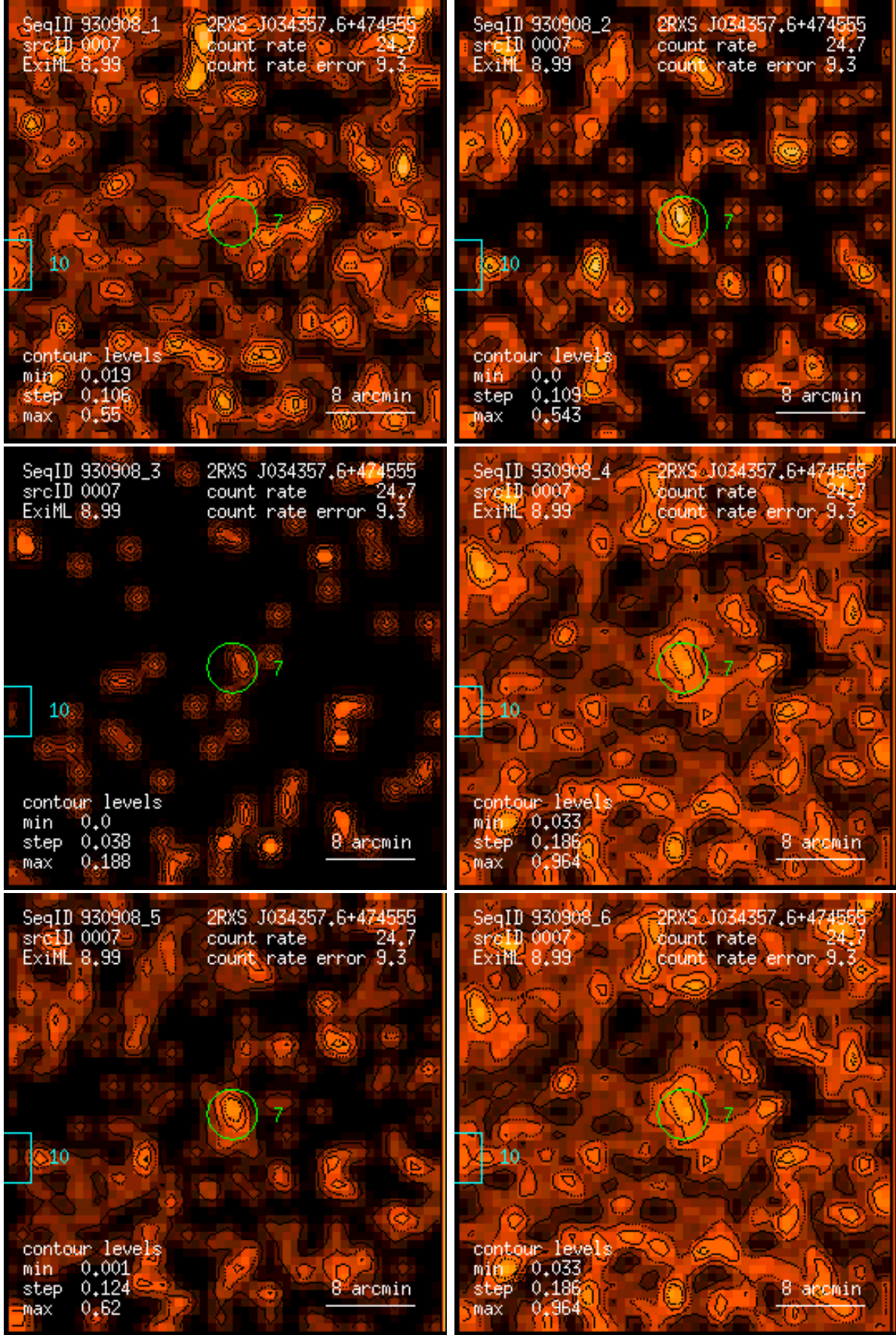
Figure 7: RASS 930908: detection 0007: band rate images, Gaussian filter: (1) PSPC channels 11 – 41, (2) 52 – 90, (3) 91 – 201, (4) 11 – 235, (5) 52 – 201, (6) 11 – 201. Broad band rates in counts/ks. Band rate contour levels in counts/ks/arcmin 2 .
