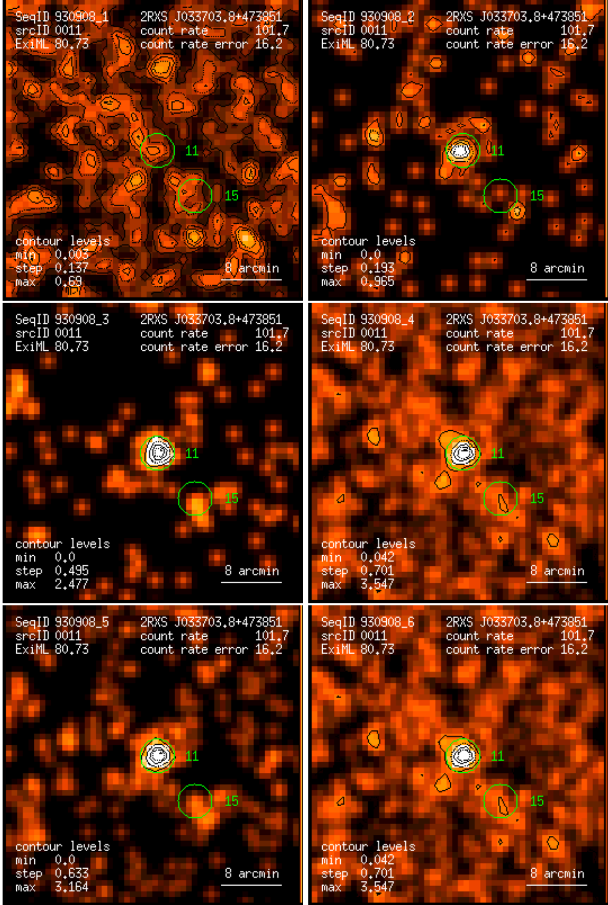
Figure 11: RASS 930908: detection 0011: band rate images, Gaussian filter: (1) PSPC channels 11 – 41, (2) 52 – 90, (3) 91 – 201, (4) 11 – 235, (5) 52 – 201, (6) 11 – 201. Broad band rates in counts/ks. Band rate contour levels in counts/ks/arcmin 2 .
