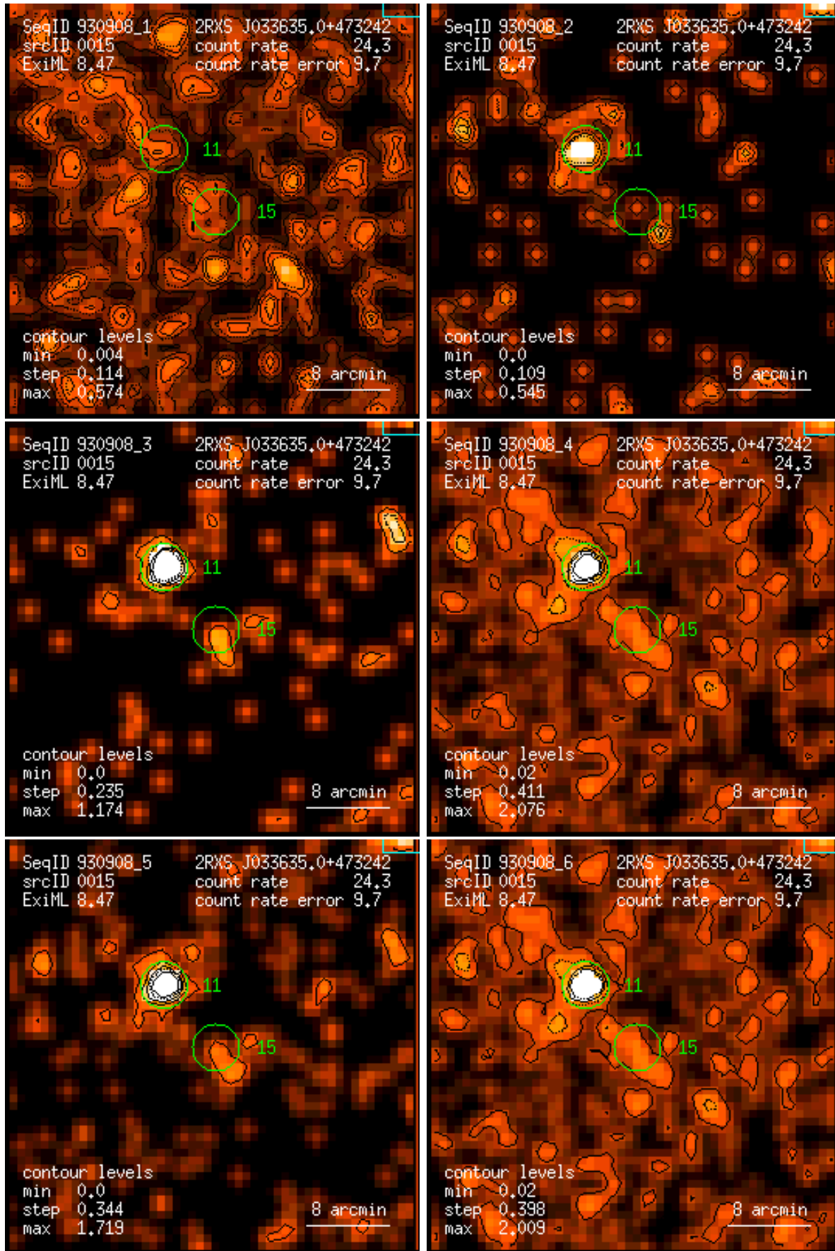
Figure 15: RASS 930908: detection 0015: band rate images, Gaussian filter: (1) PSPC channels 11 – 41, (2) 52 – 90, (3) 91 – 201, (4) 11 – 235, (5) 52 – 201, (6) 11 – 201. Broad band rates in counts/ks. Band rate contour levels in counts/ks/arcmin 2 .
