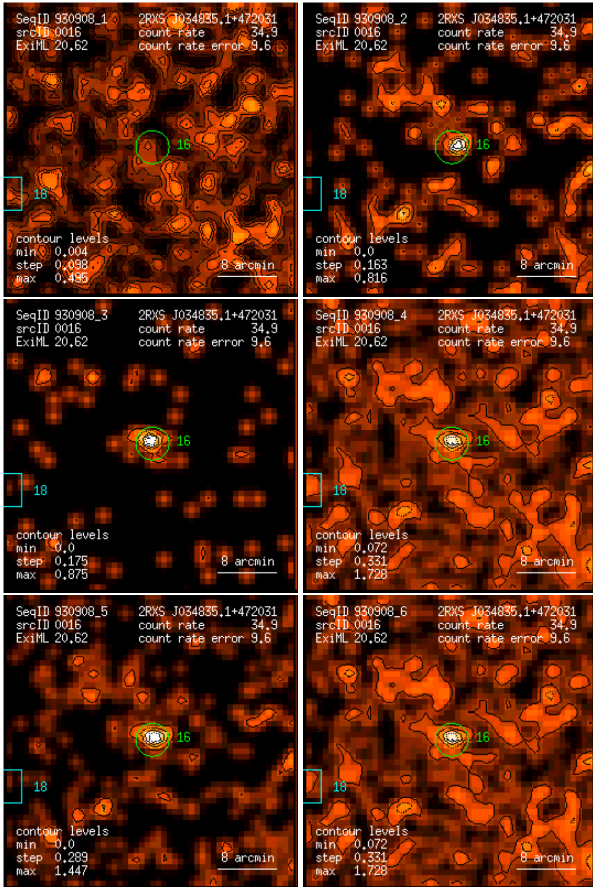
Figure 16: RASS 930908: detection 0016: band rate images, Gaussian filter: (1) PSPC channels 11 – 41, (2) 52 – 90, (3) 91 – 201, (4) 11 – 235, (5) 52 – 201, (6) 11 – 201. Broad band rates in counts/ks. Band rate contour levels in counts/ks/arcmin 2 .
