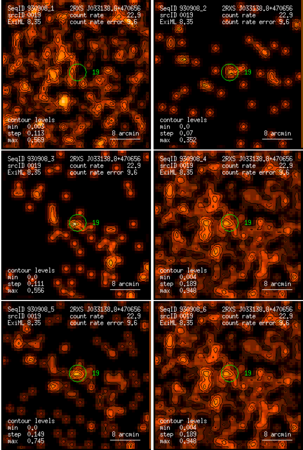
Figure 19: RASS 930908: detection 0019: band rate images, Gaussian filter: (1) PSPC channels 11 – 41, (2) 52 – 90, (3) 91 – 201, (4) 11 – 235, (5) 52 – 201, (6) 11 – 201. Broad band rates in counts/ks. Band rate contour levels in counts/ks/arcmin 2 .
