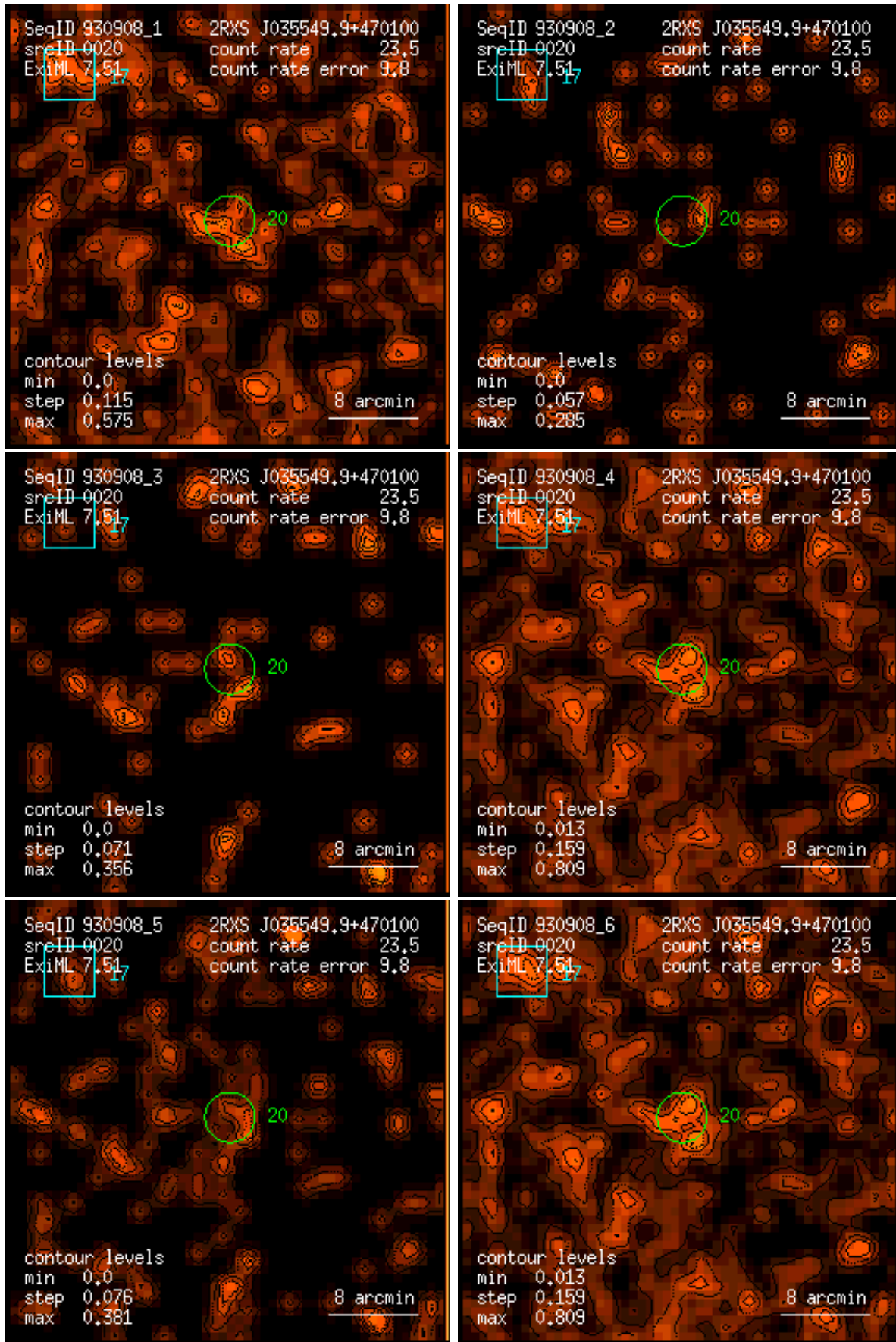
Figure 20: RASS 930908: detection 0020: band rate images, Gaussian filter: (1) PSPC channels 11 – 41, (2) 52 – 90, (3) 91 – 201, (4) 11 – 235, (5) 52 – 201, (6) 11 – 201. Broad band rates in counts/ks. Band rate contour levels in counts/ks/arcmin 2 .
